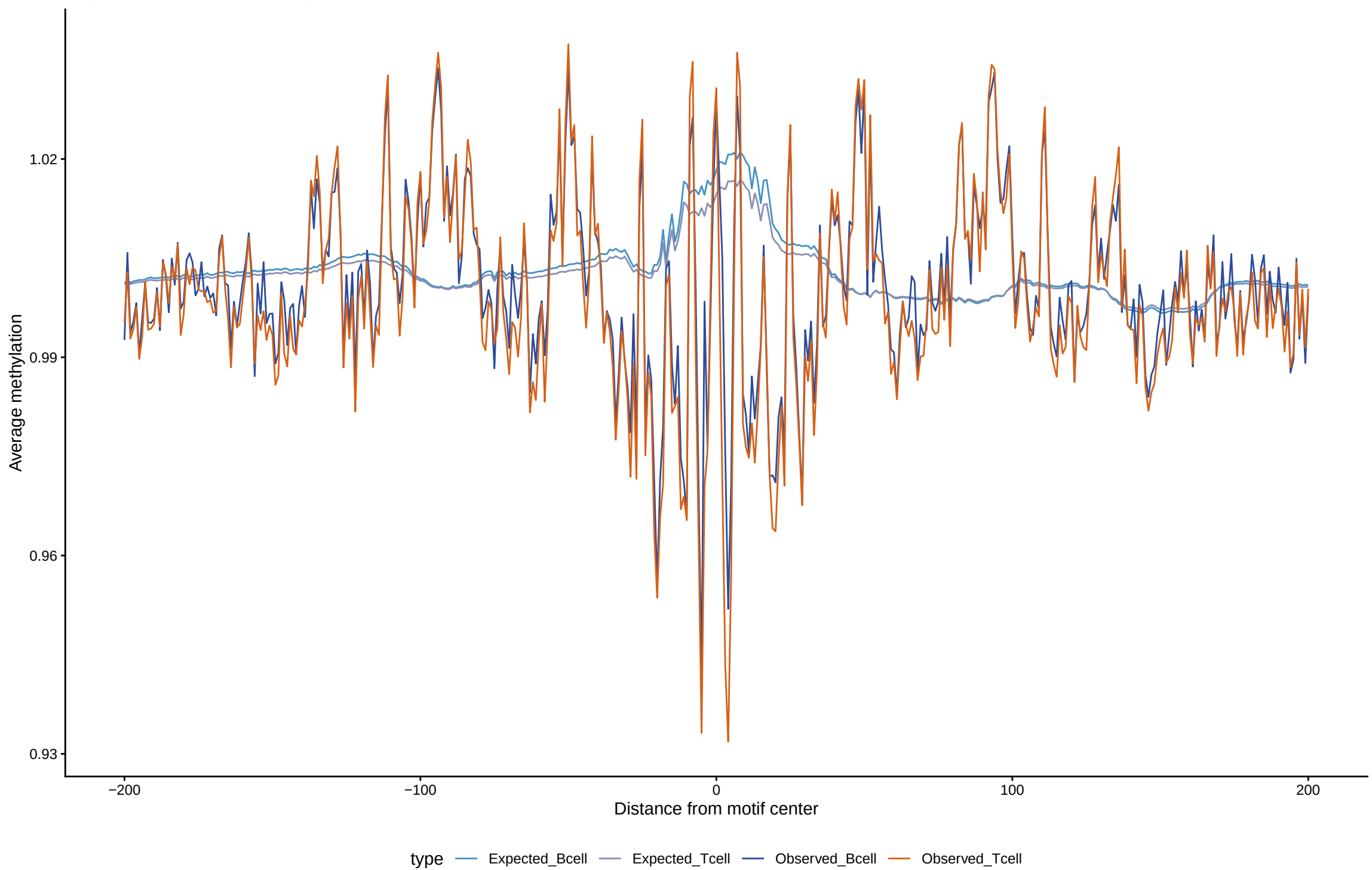
Expected vs observed footprints for ATF4
