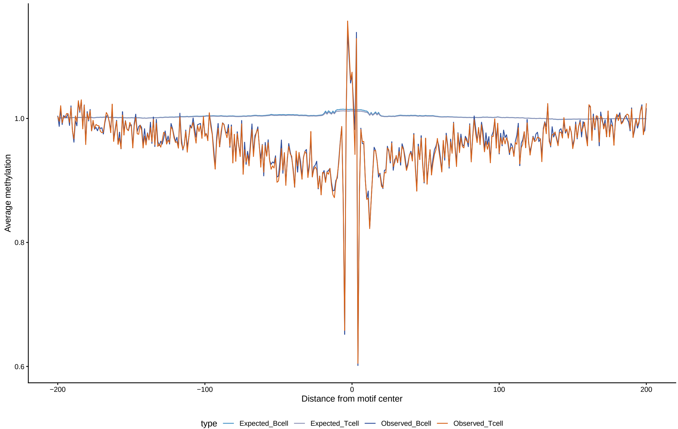
Expected vs observed footprints for ATF7
