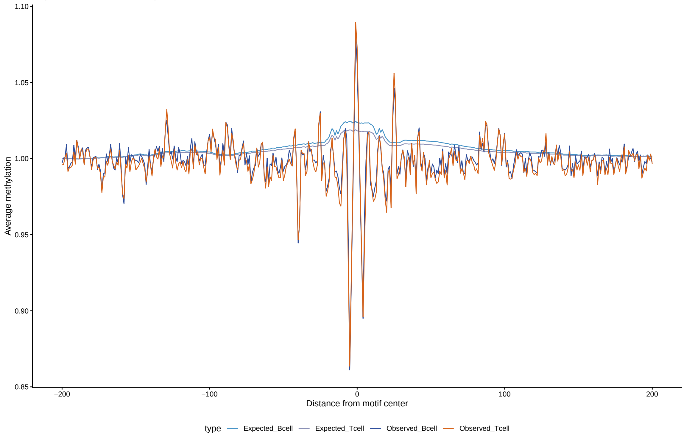
Expected vs observed footprints for CEBPA
