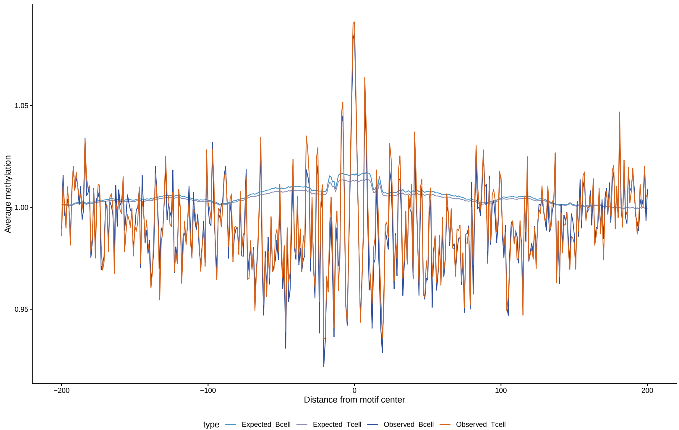
Expected vs observed footprints for CEBPB
