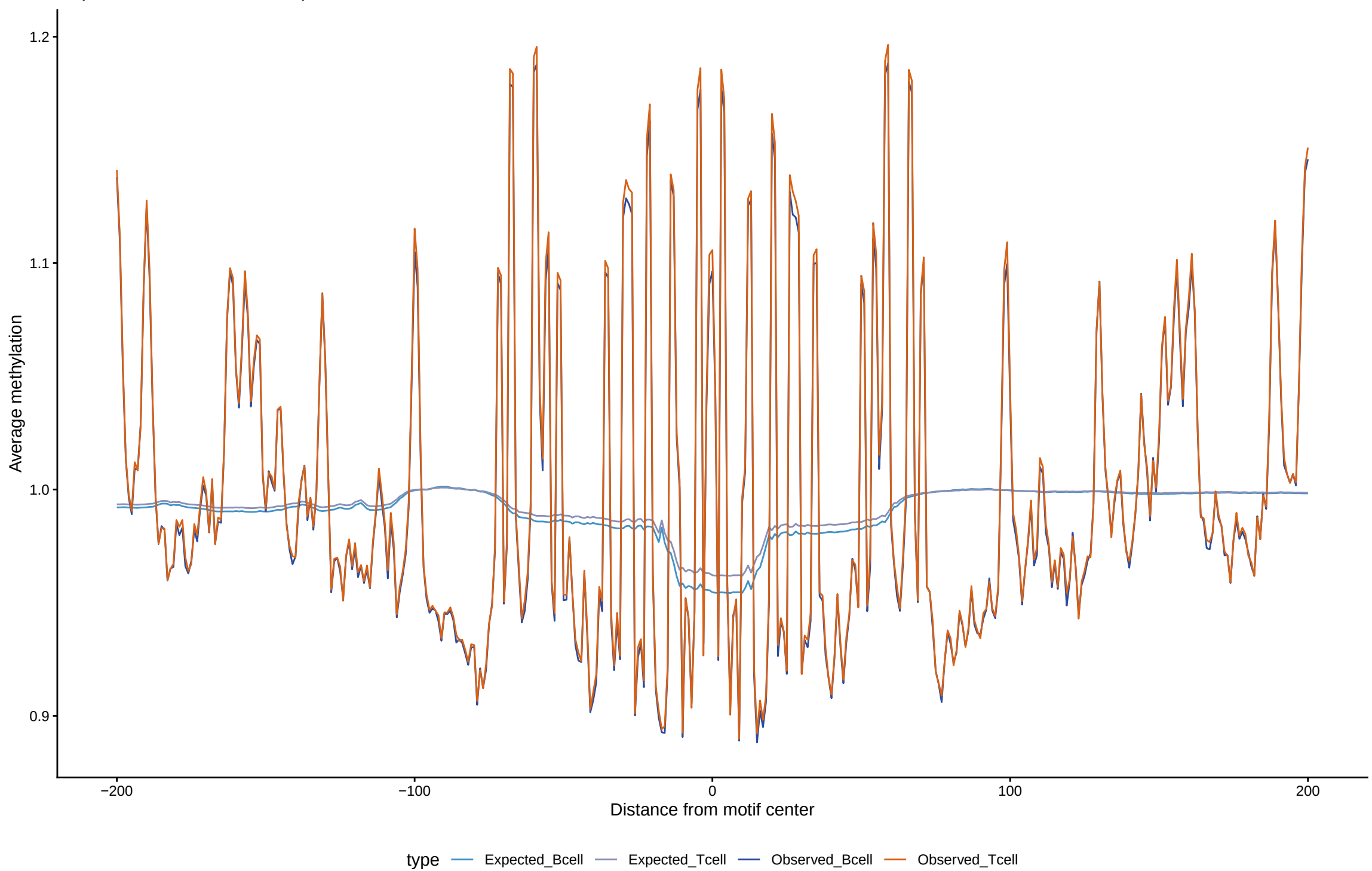
Expected vs observed footprints for CTCFL
