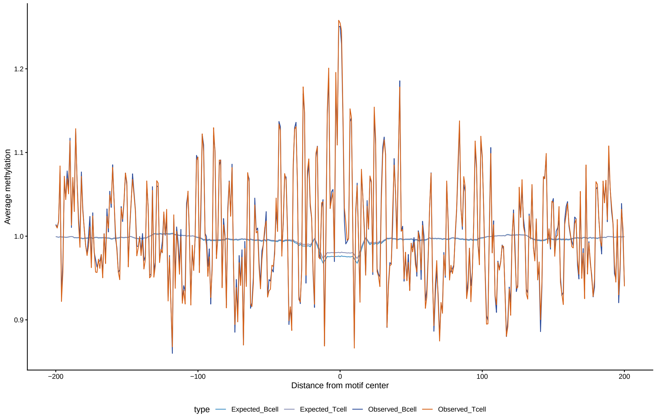
Expected vs observed footprints for E2F1
