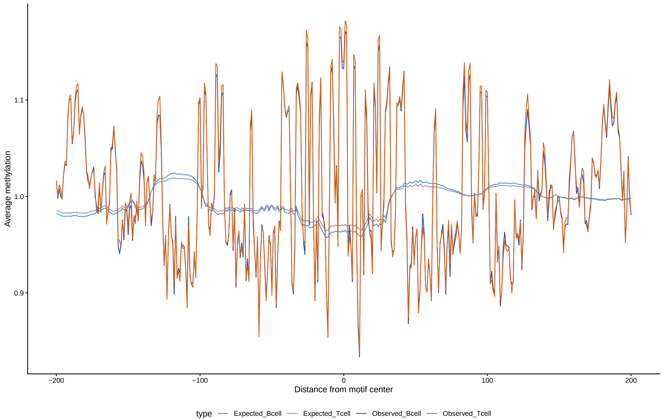
Expected vs observed footprints for E2F2
