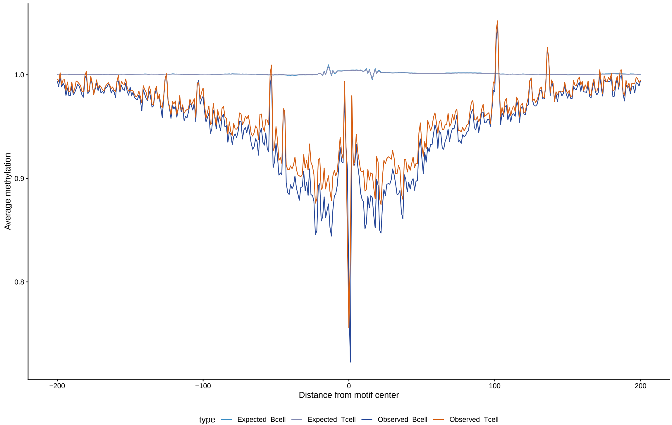
Expected vs observed footprints for ELF3
