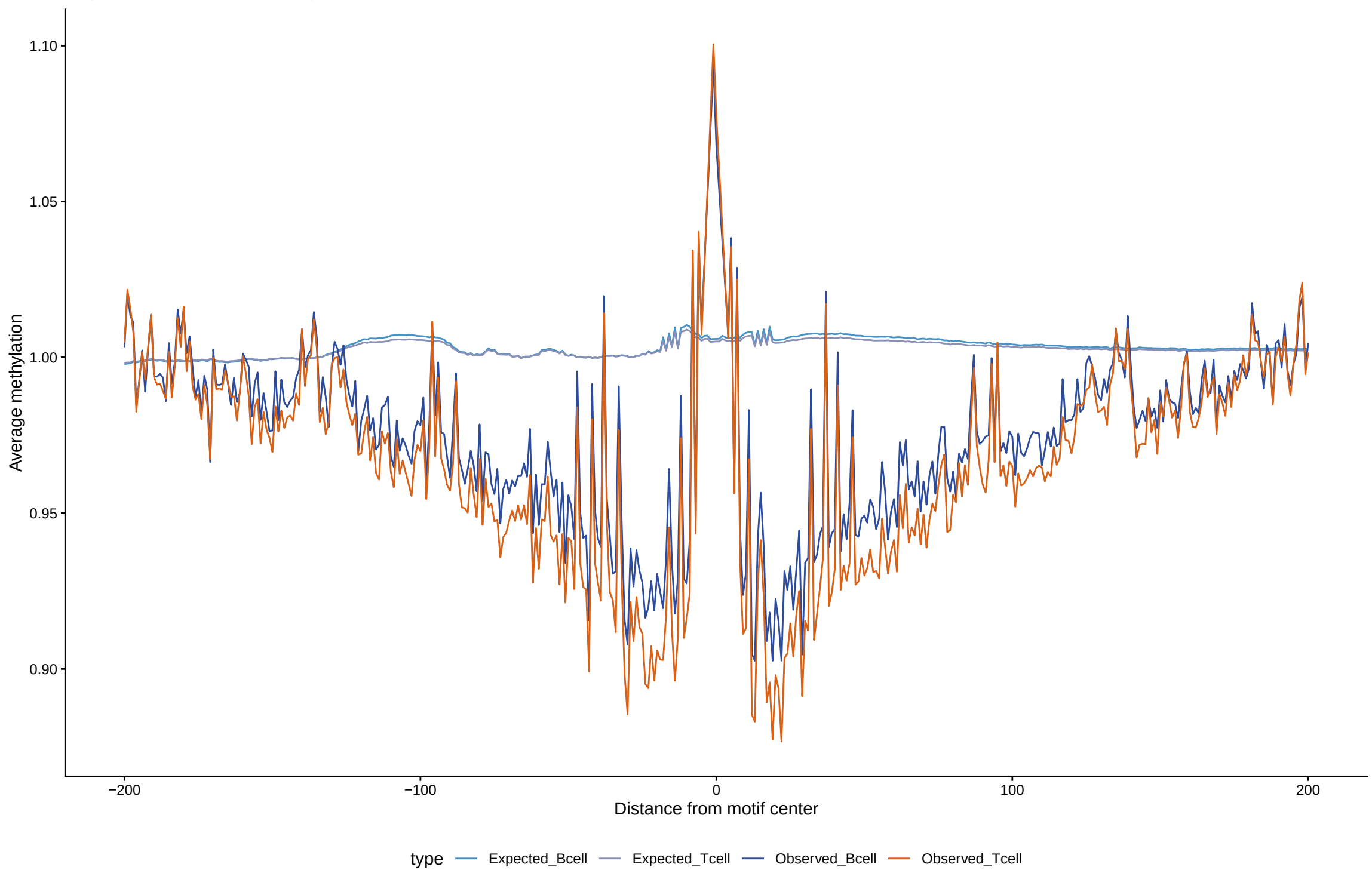
Expected vs observed footprints for FOS::JUND
