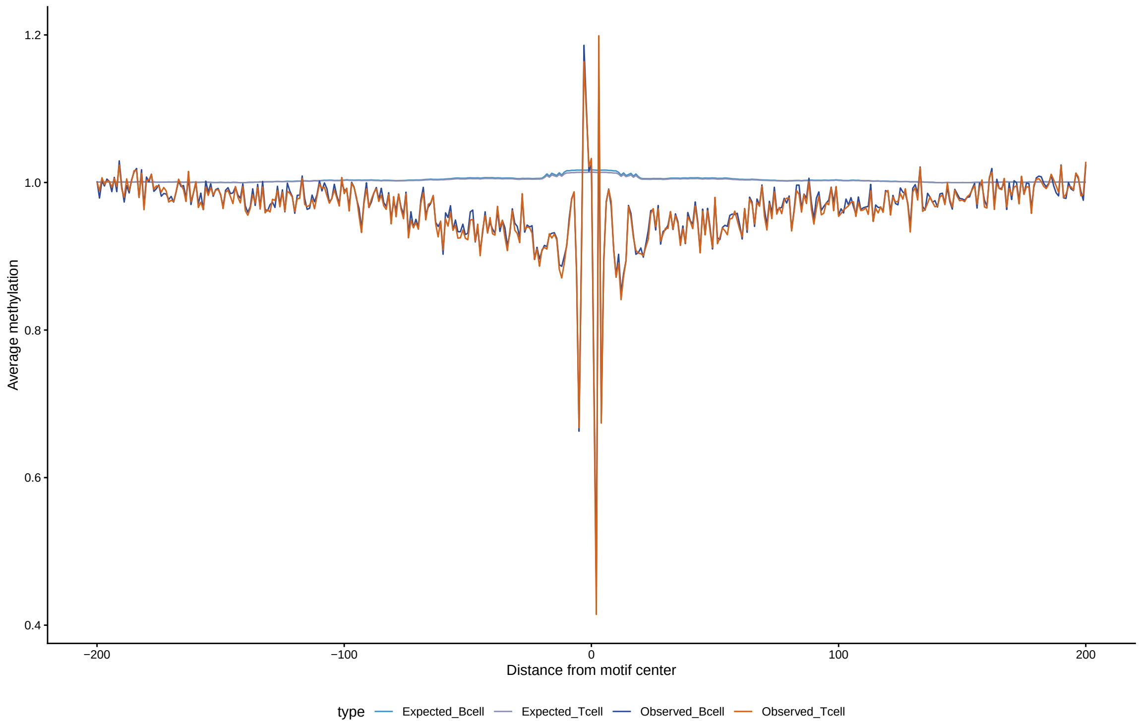
Expected vs observed footprints for FOSL2::JUNB(var.2)
