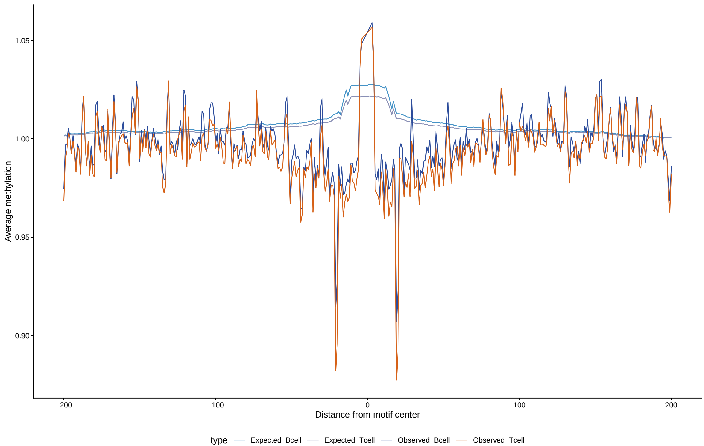
Expected vs observed footprints for FOXG1
