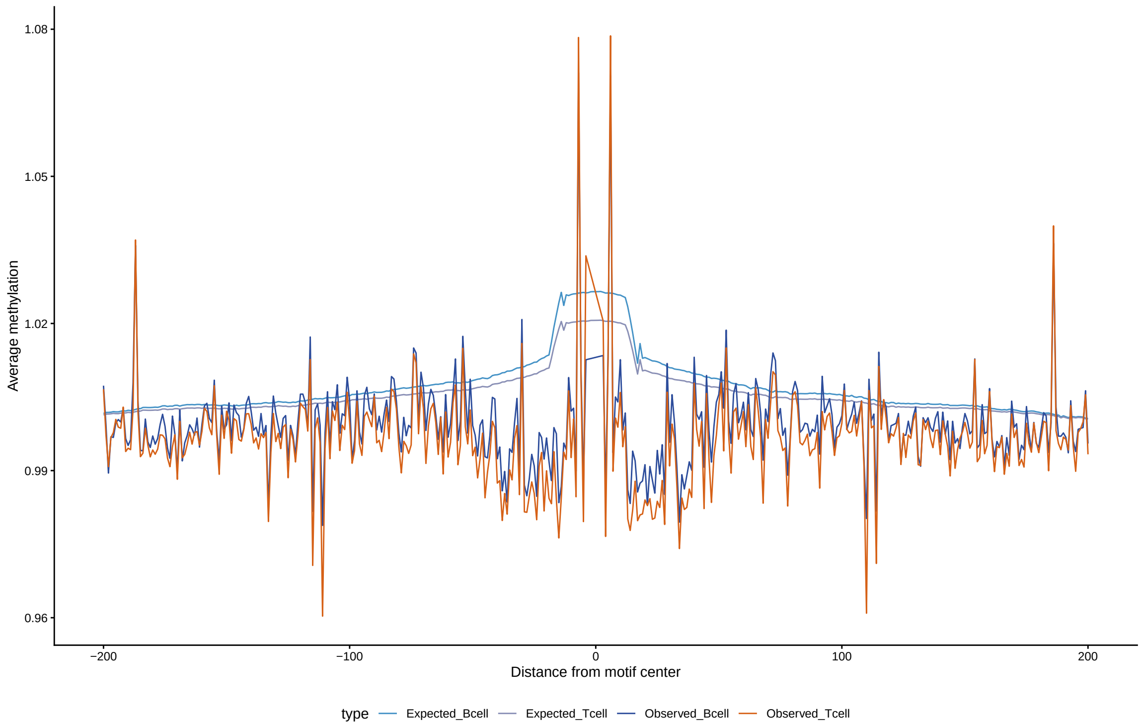
Expected vs observed footprints for FOXL1
