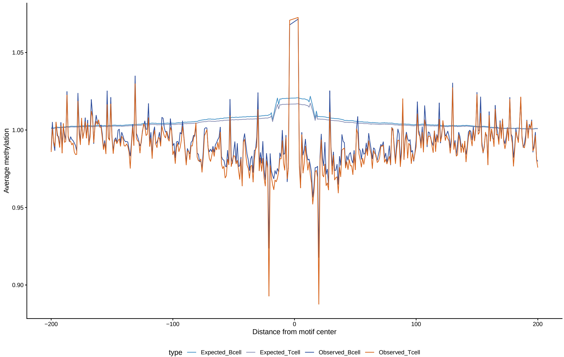
Expected vs observed footprints for FOXO6
