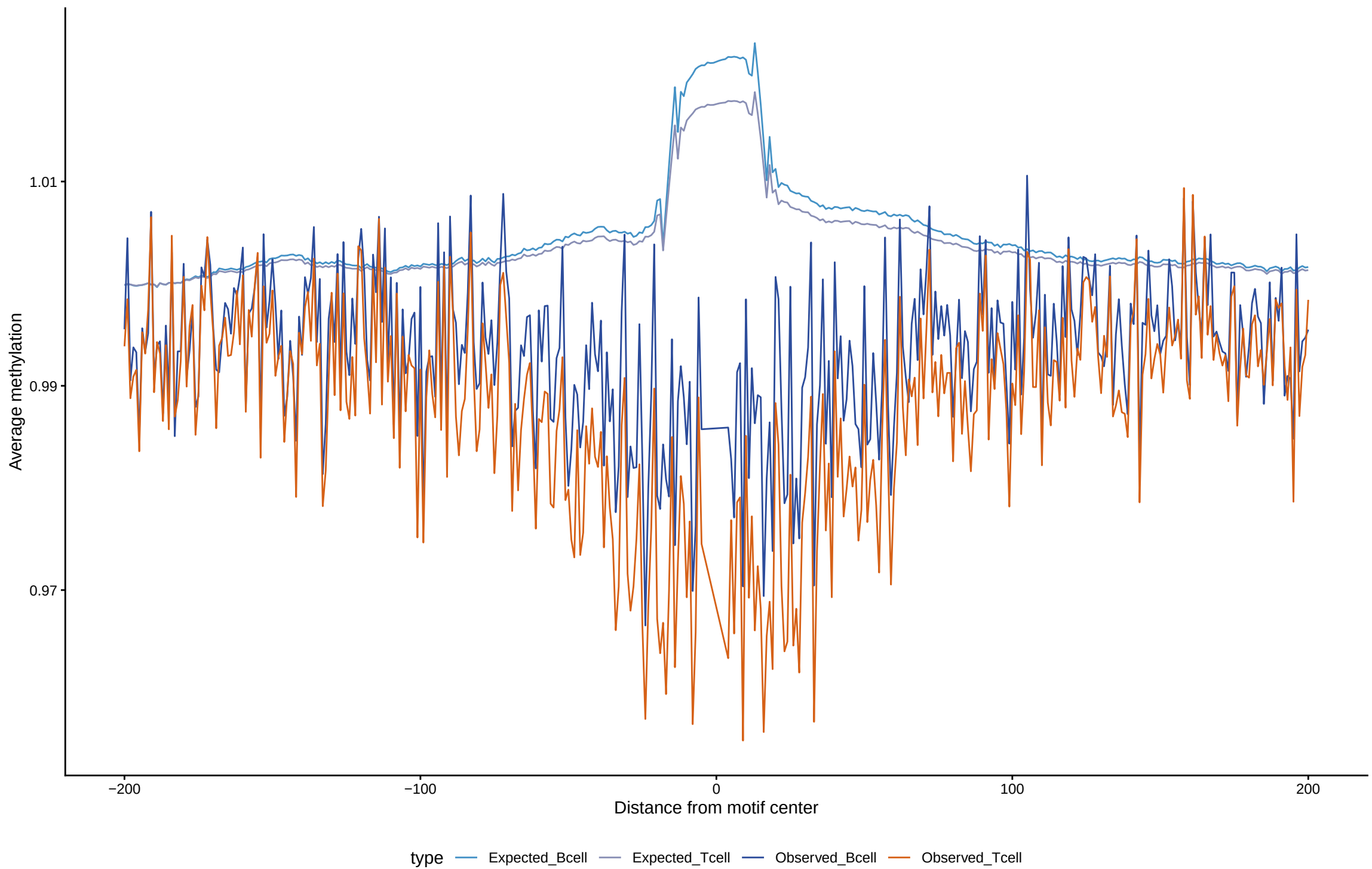
Expected vs observed footprints for GATA2
