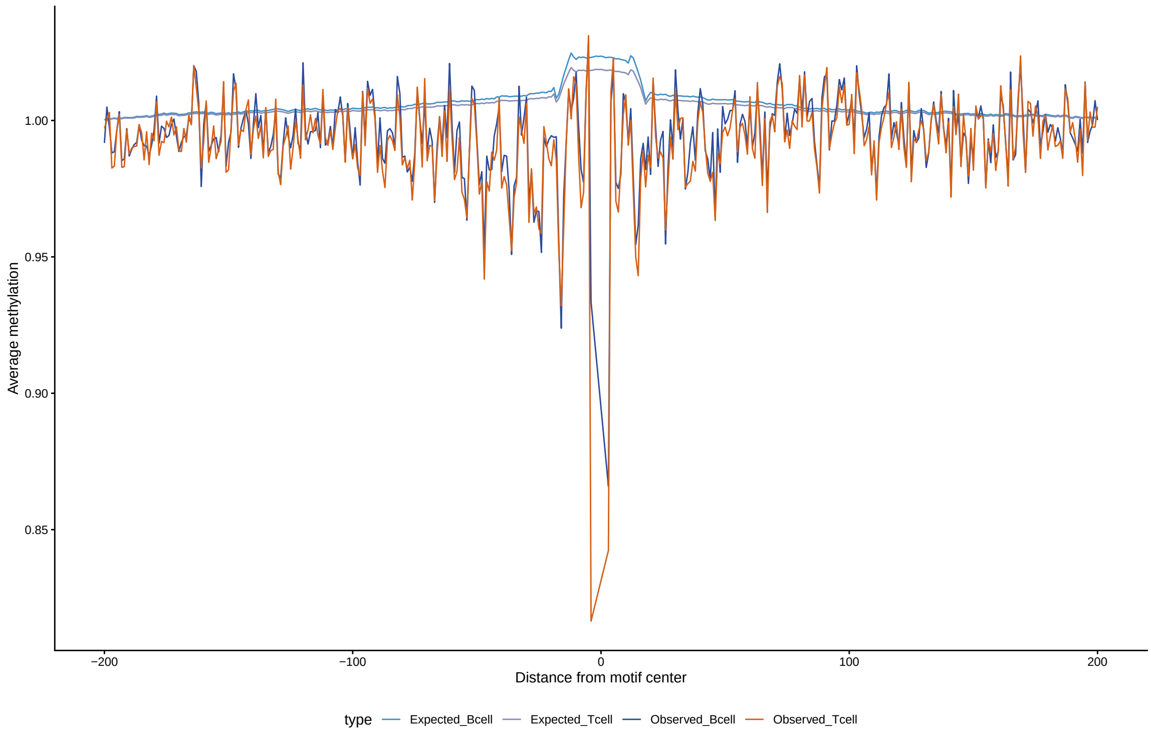
Expected vs observed footprints for GBX1
