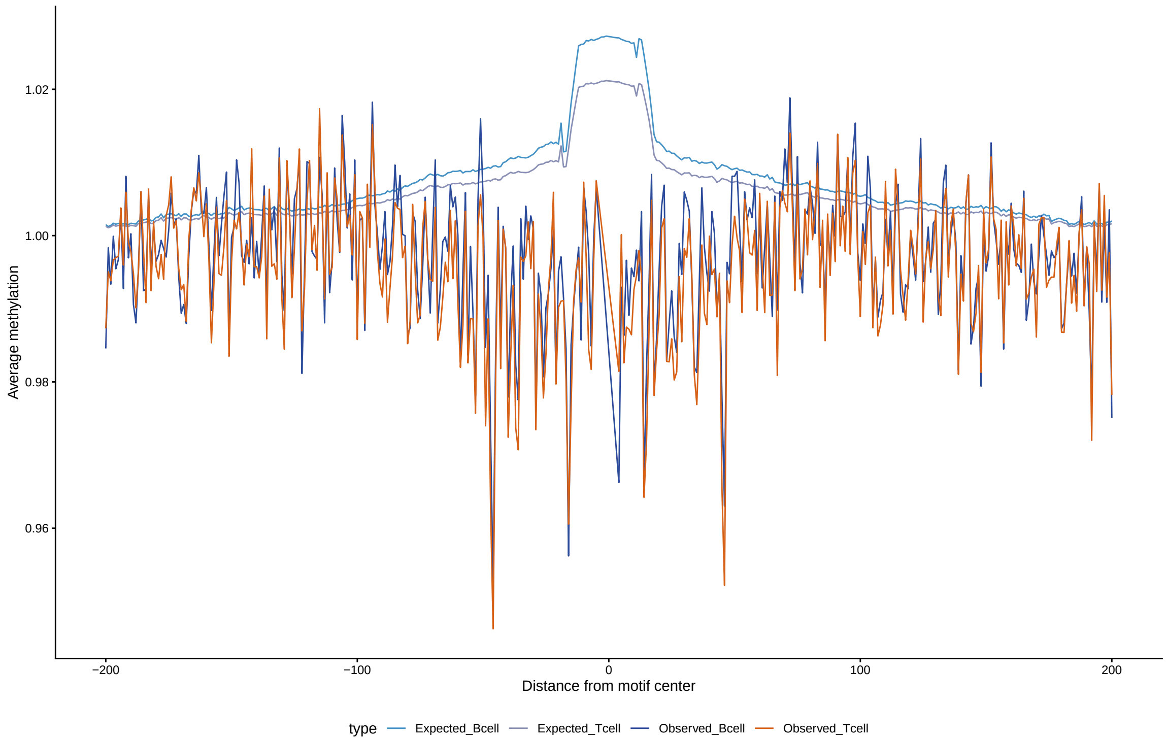
Expected vs observed footprints for GBX2
