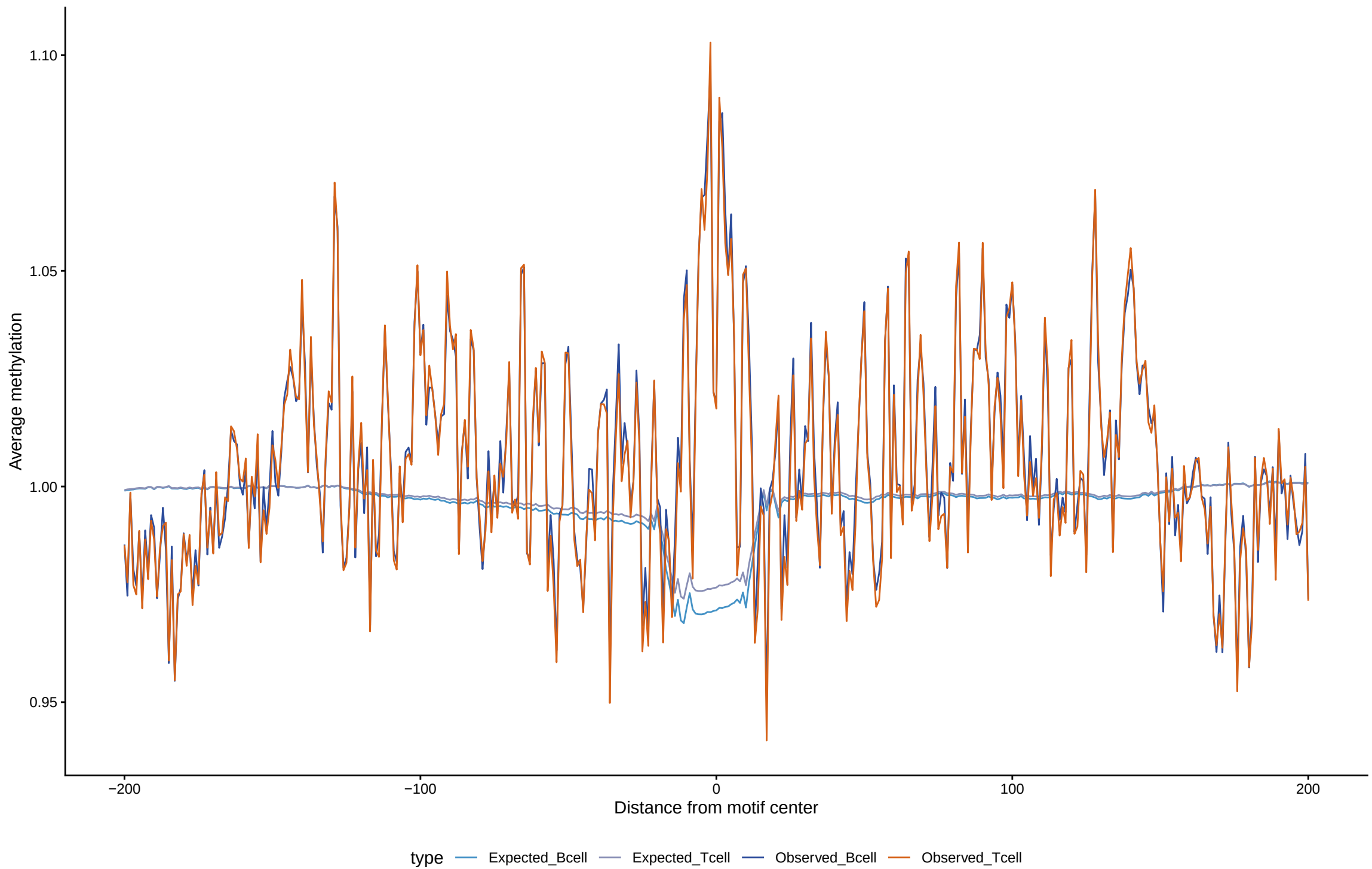
Expected vs observed footprints for GLIS1
