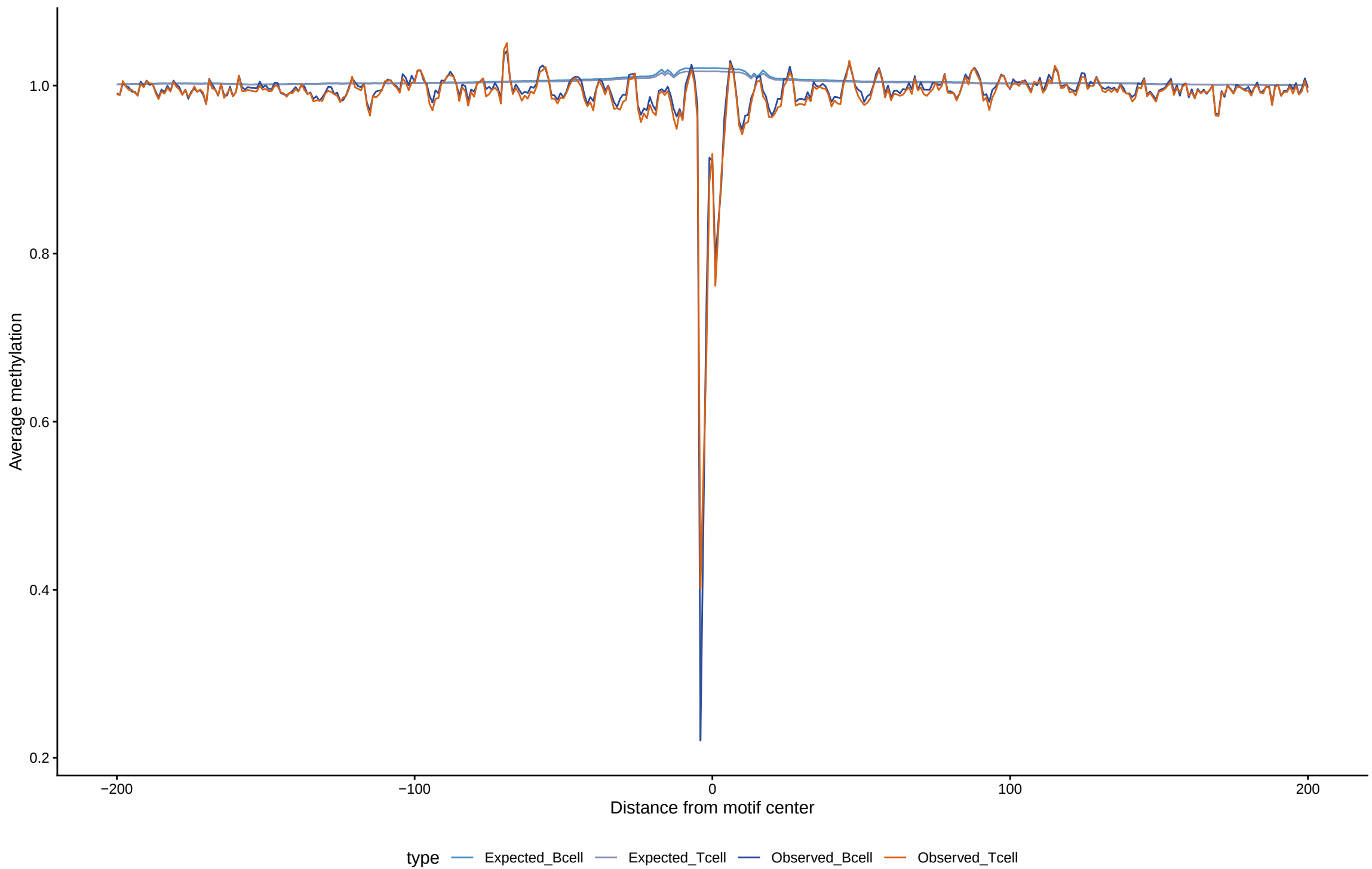
Expected vs observed footprints for GRHL2
