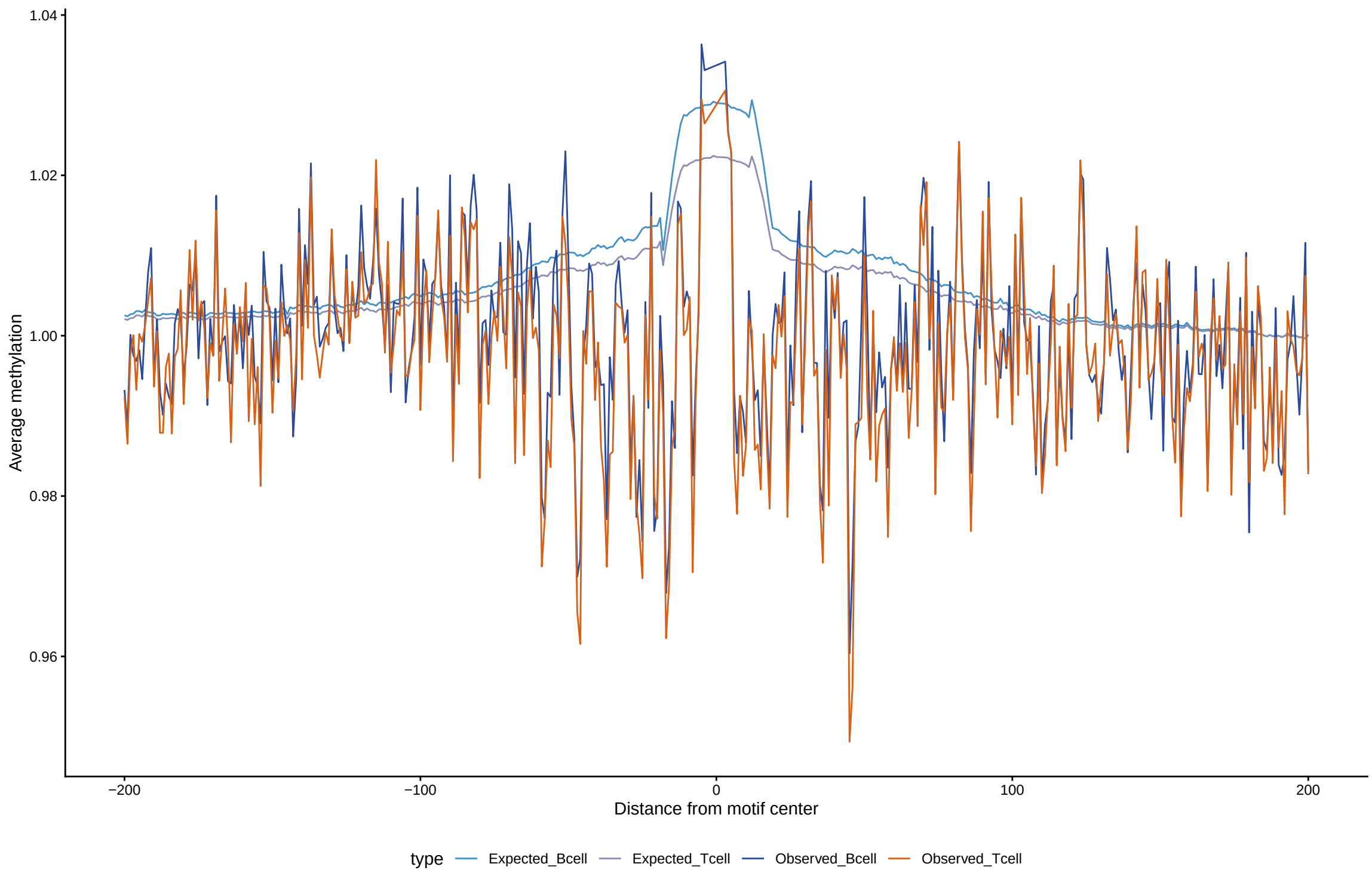
Expected vs observed footprints for GSX2
