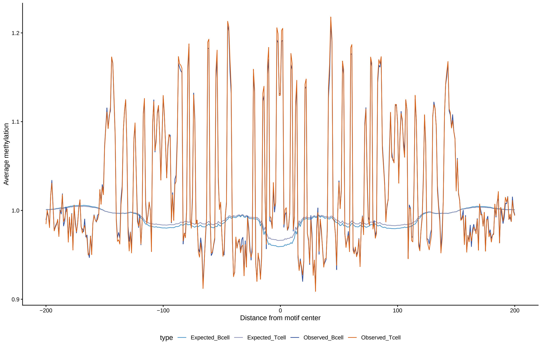
Expected vs observed footprints for HES1
