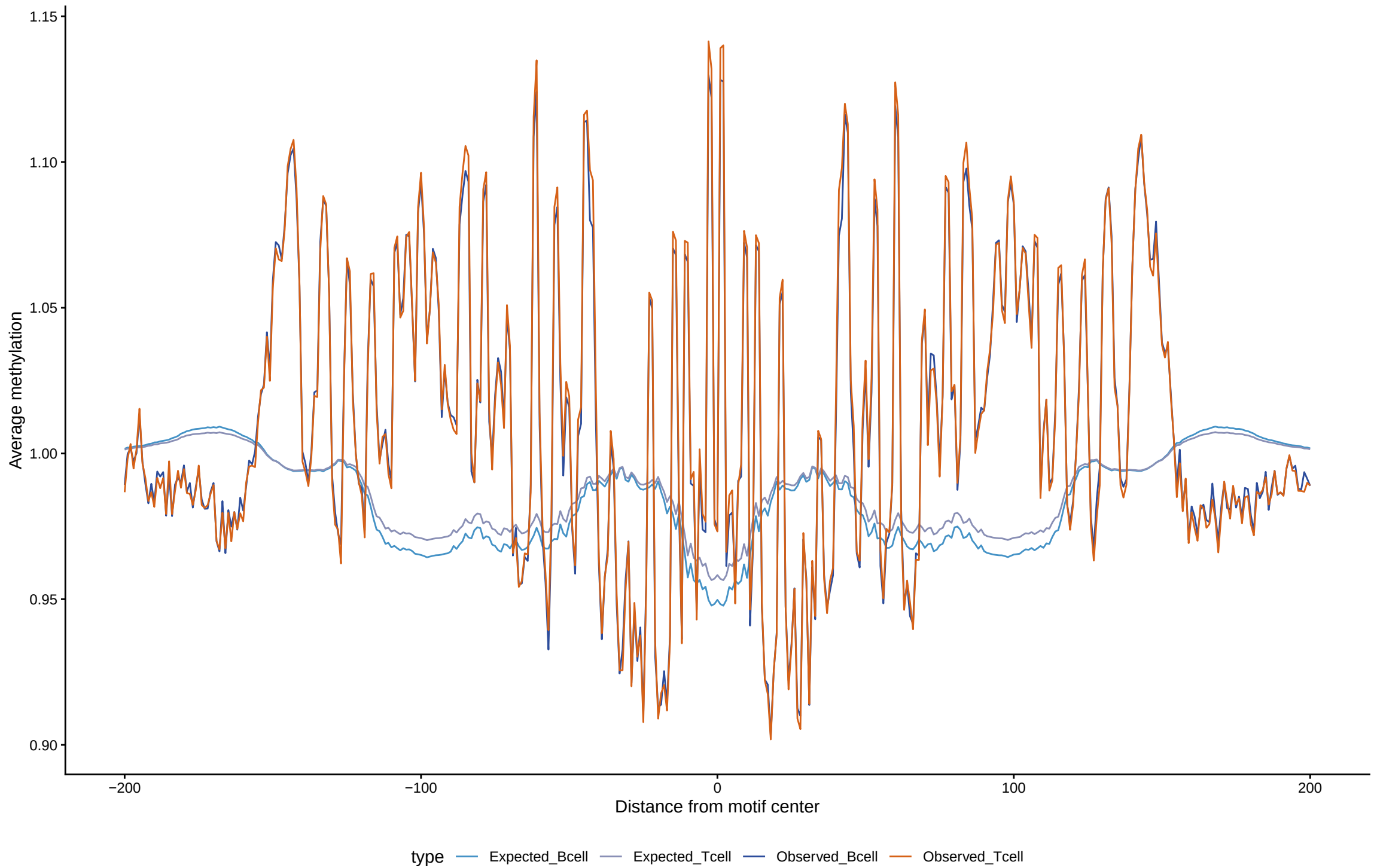
Expected vs observed footprints for HES7
