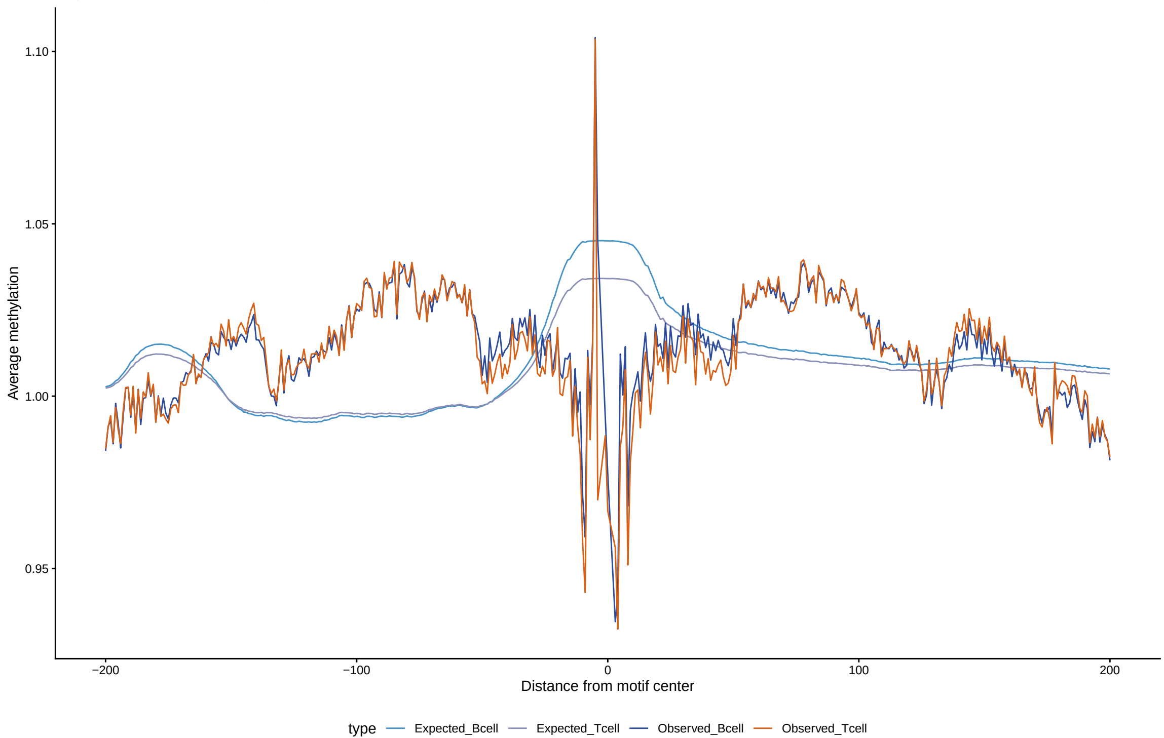
Expected vs observed footprints for HNF1A
