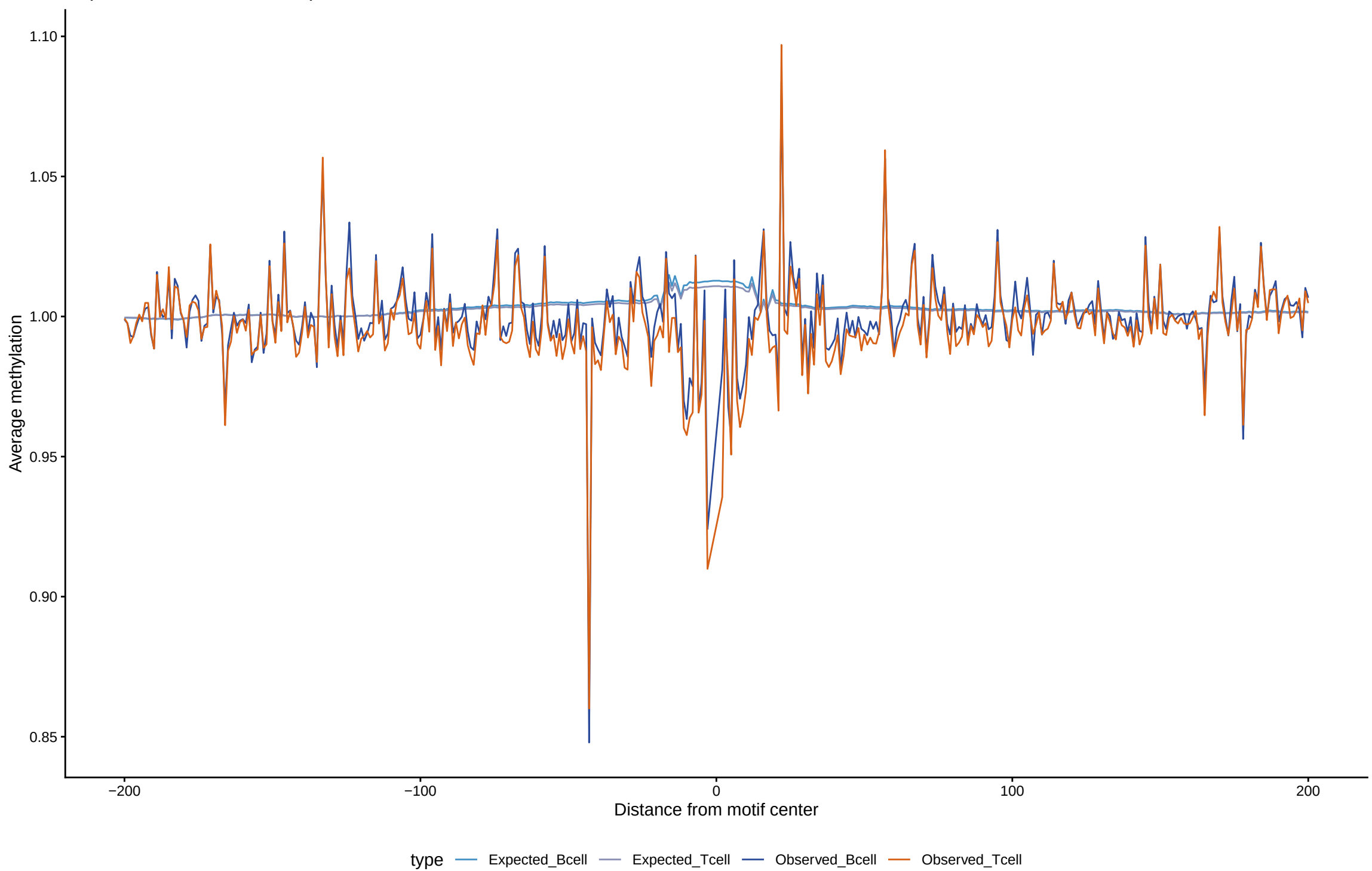
Expected vs observed footprints for HNF4A
