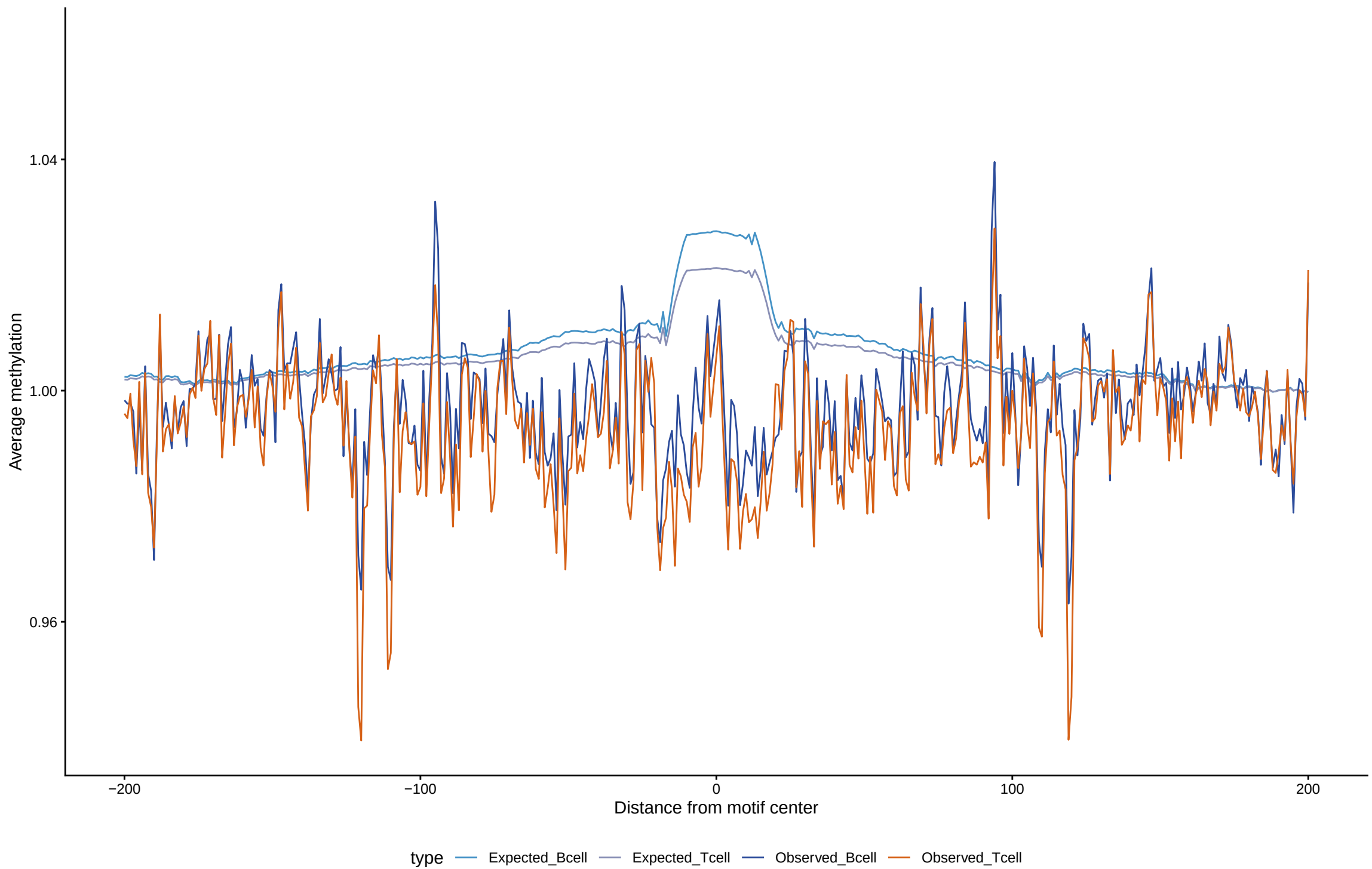
Expected vs observed footprints for HOXC10
