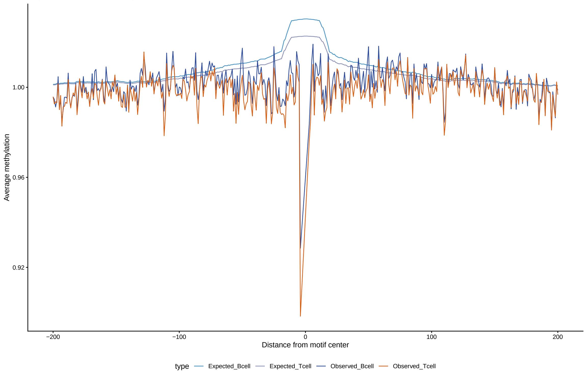
Expected vs observed footprints for HOXC4
