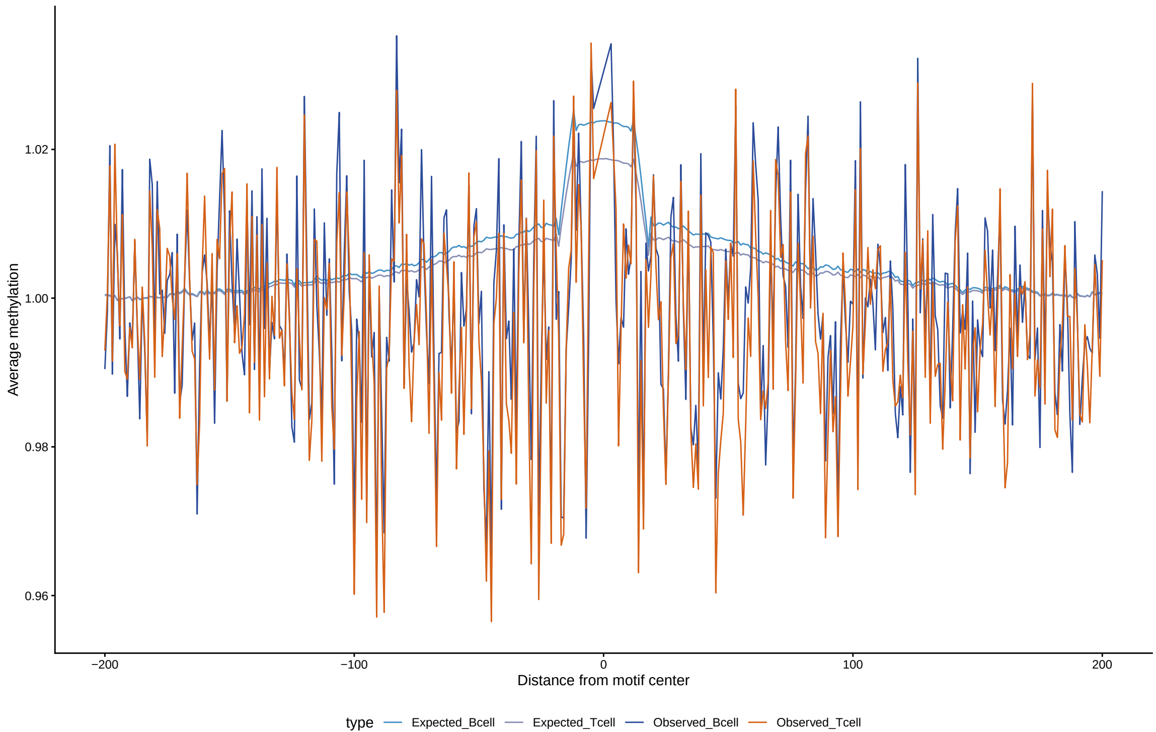
Expected vs observed footprints for HOXC8
