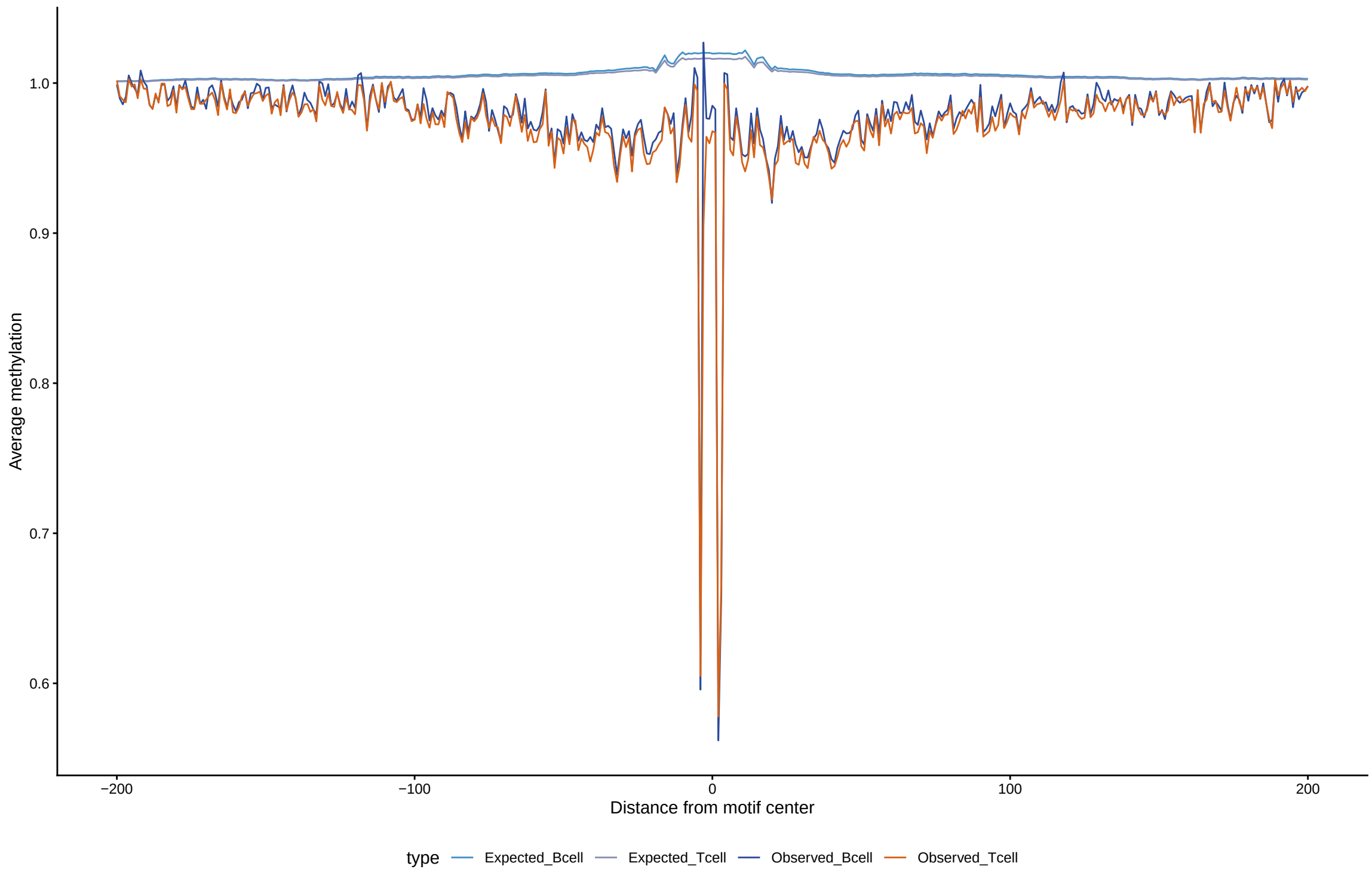
Expected vs observed footprints for IRF5
