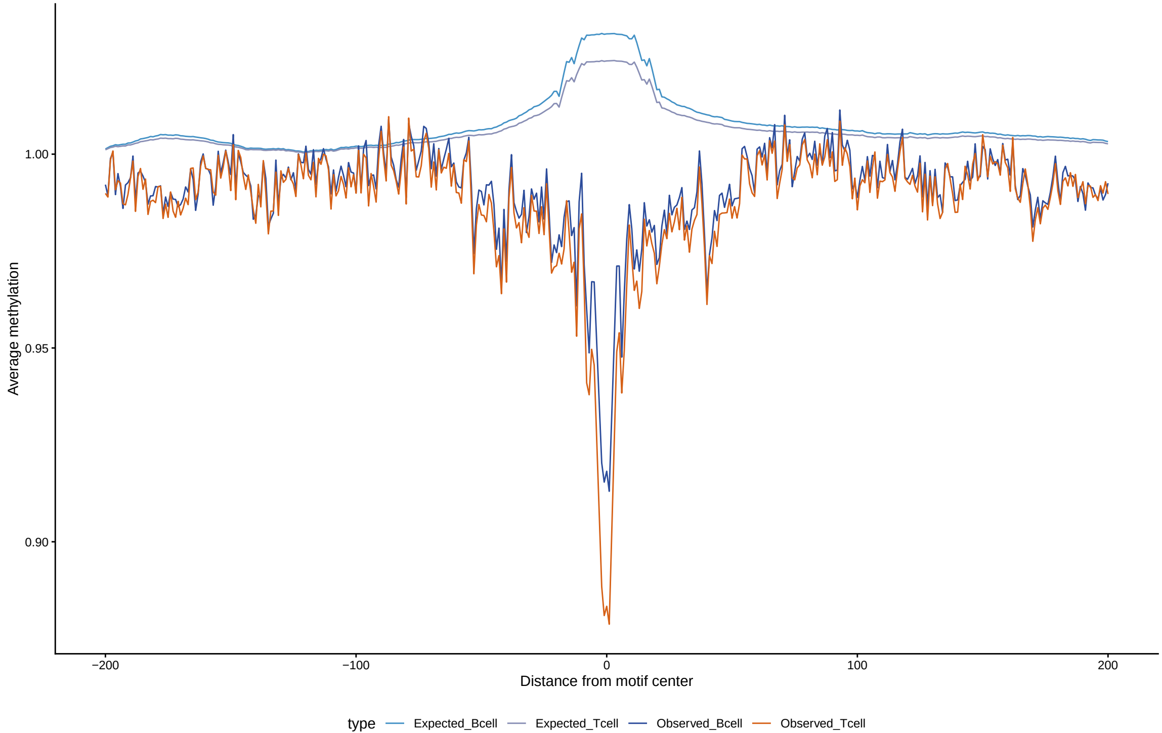
Expected vs observed footprints for IRF7
