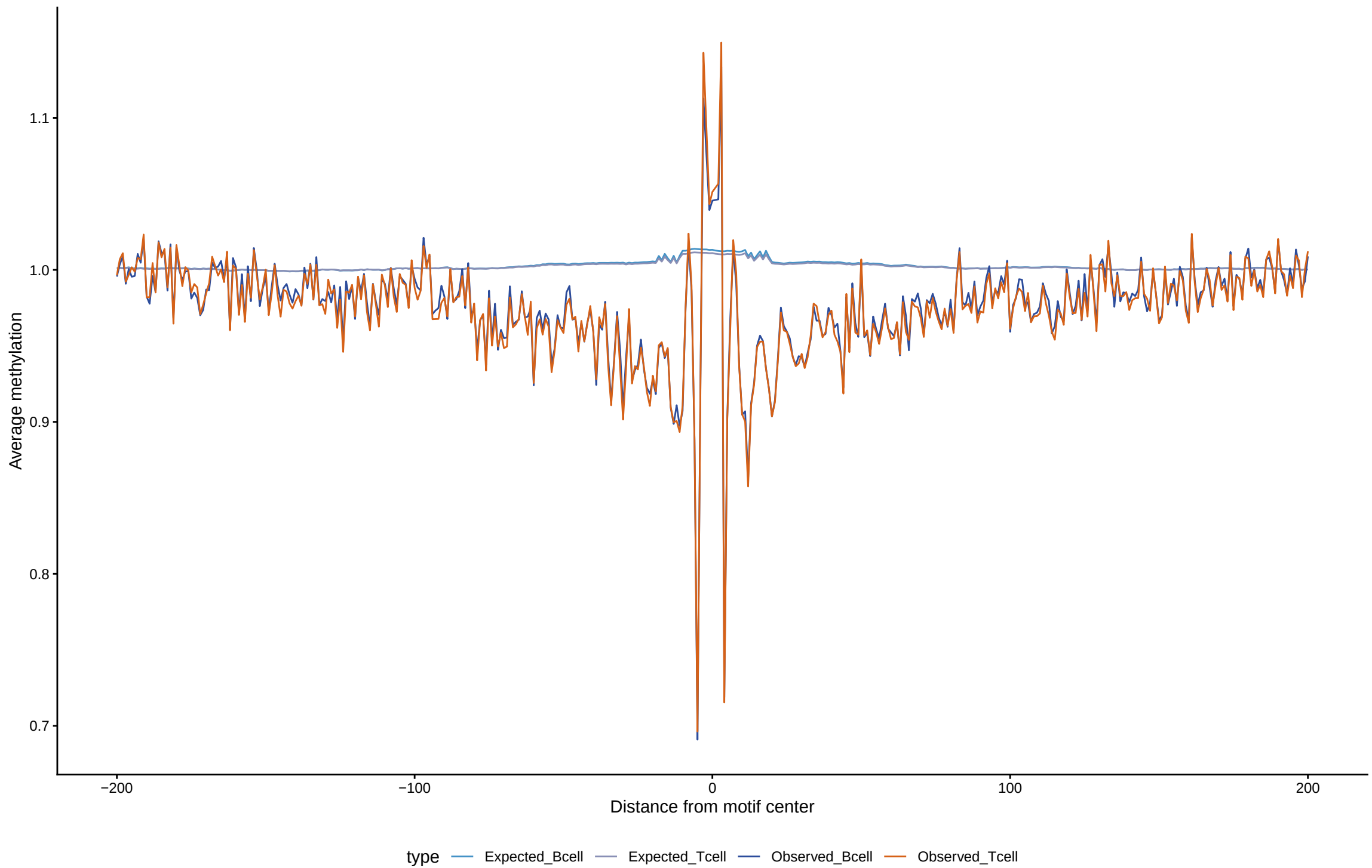
Expected vs observed footprints for JUN::JUNB(var.2)
