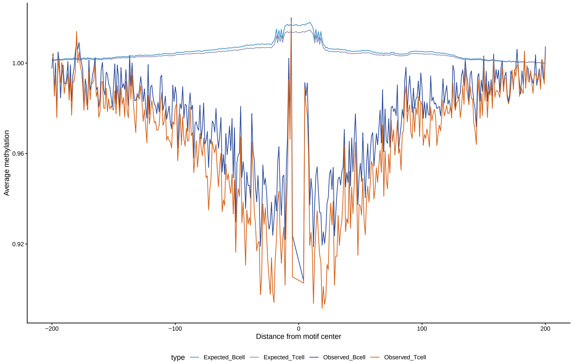
Expected vs observed footprints for JUNB
