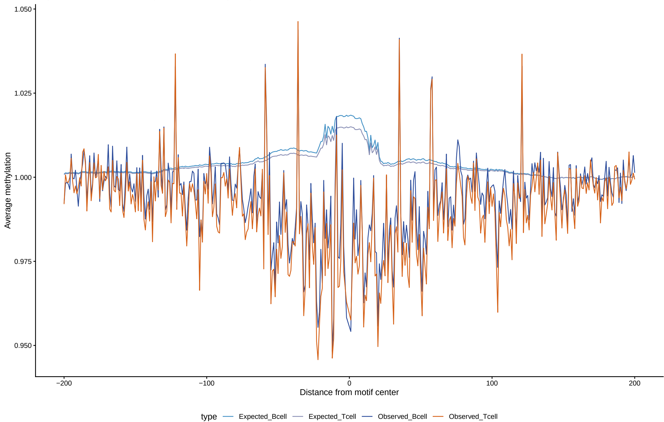
Expected vs observed footprints for JUND(var.2)
