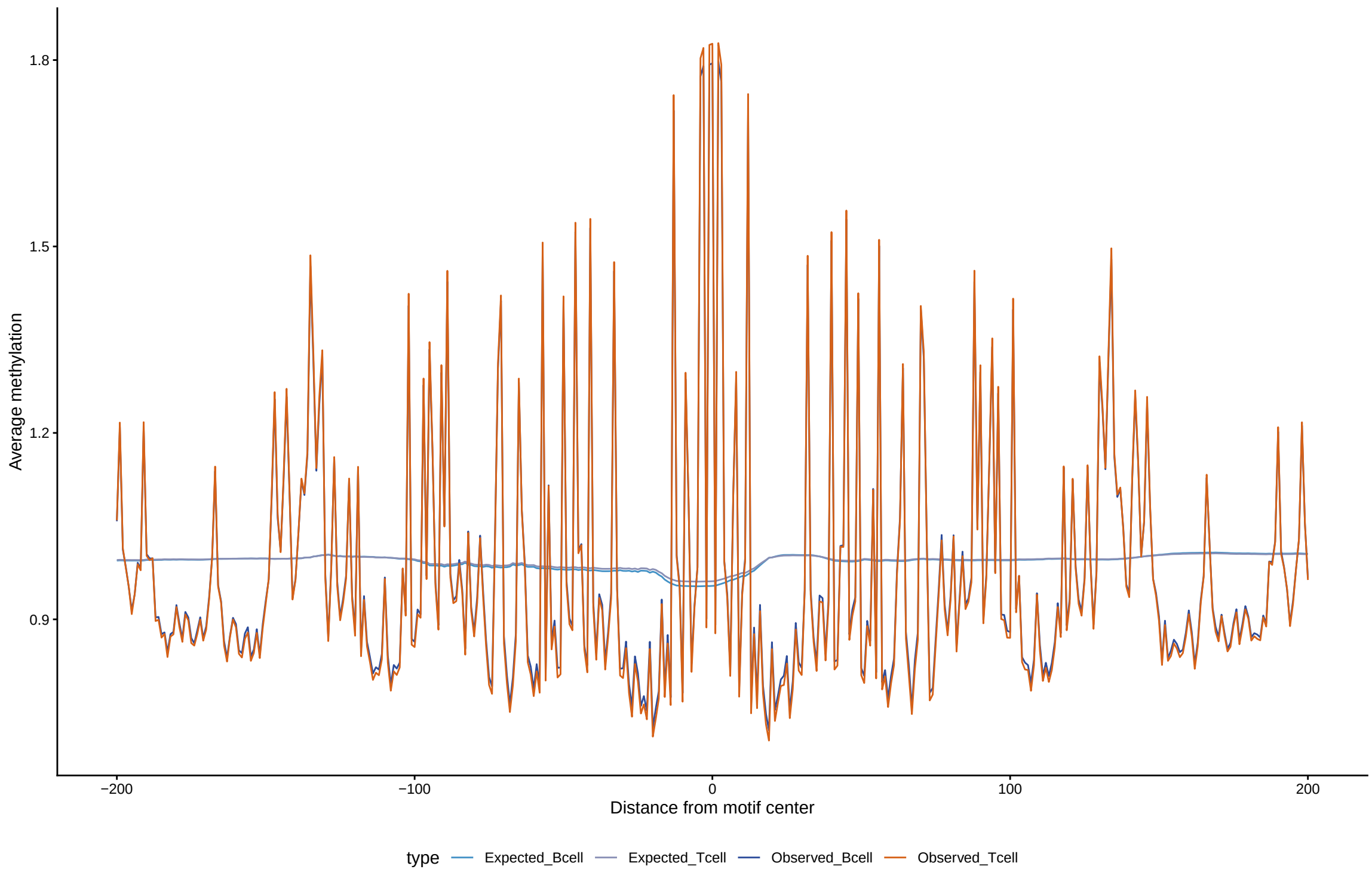
Expected vs observed footprints for KLF15
