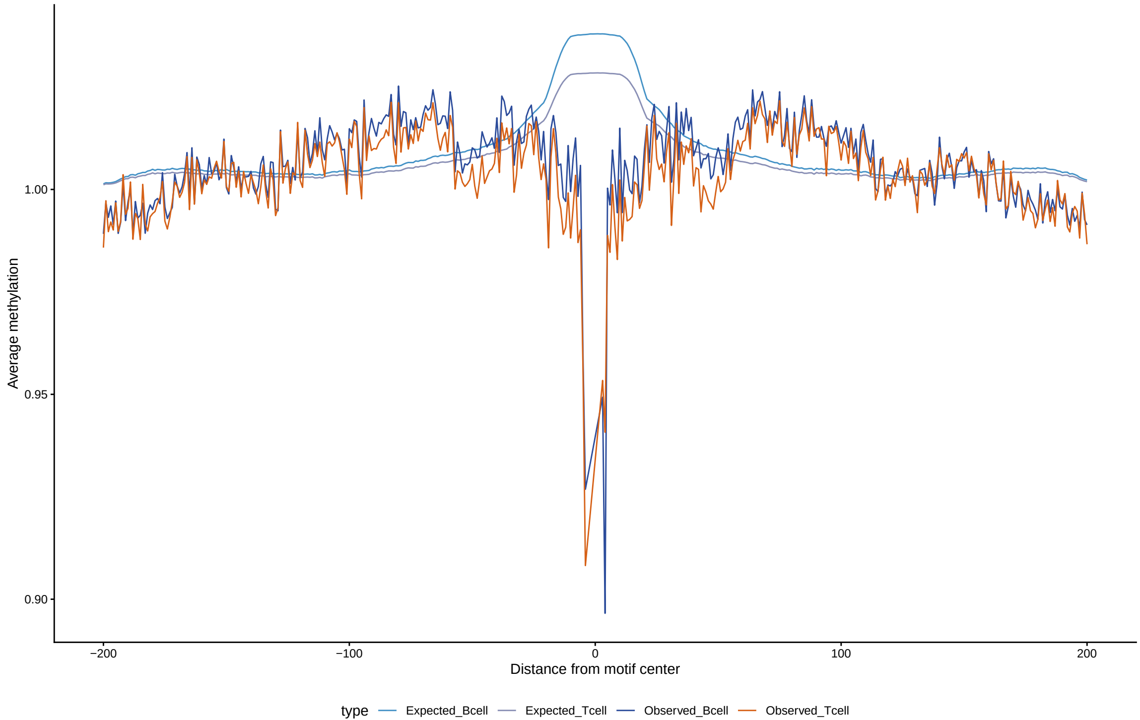
Expected vs observed footprints for LMX1B
