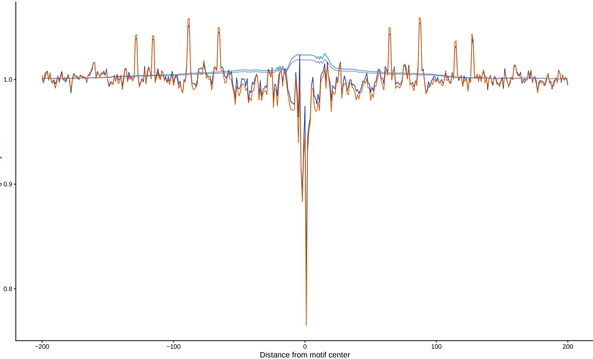
Expected vs observed footprints for MAFF
