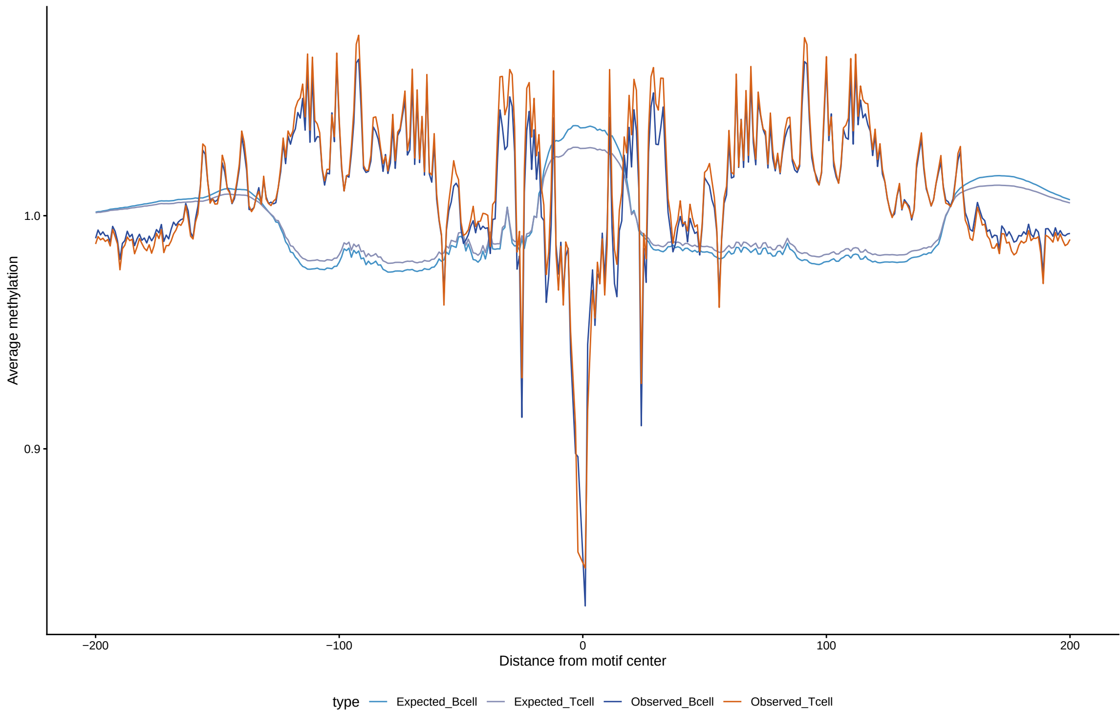
Expected vs observed footprints for MEF2C
