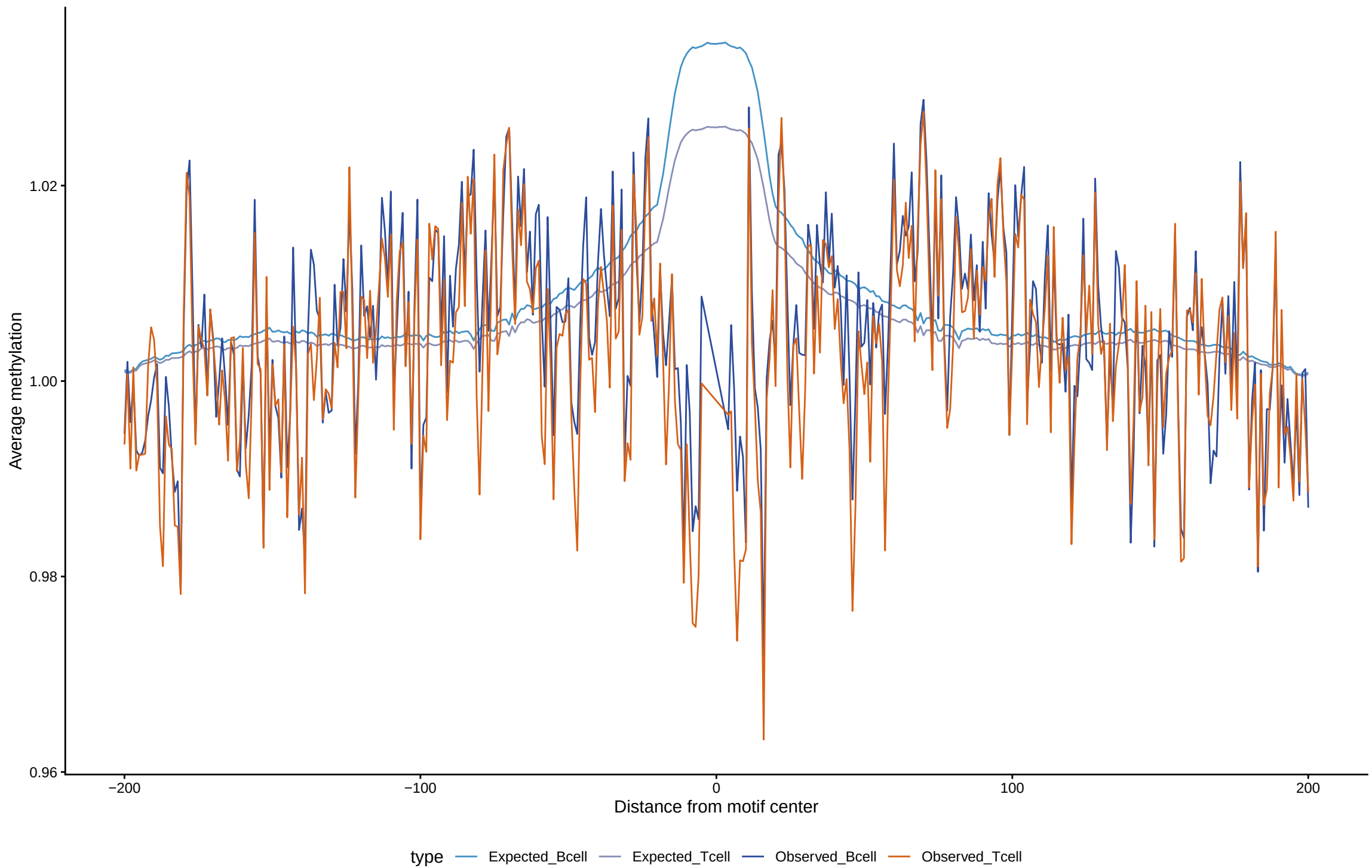
Expected vs observed footprints for MIXL1
