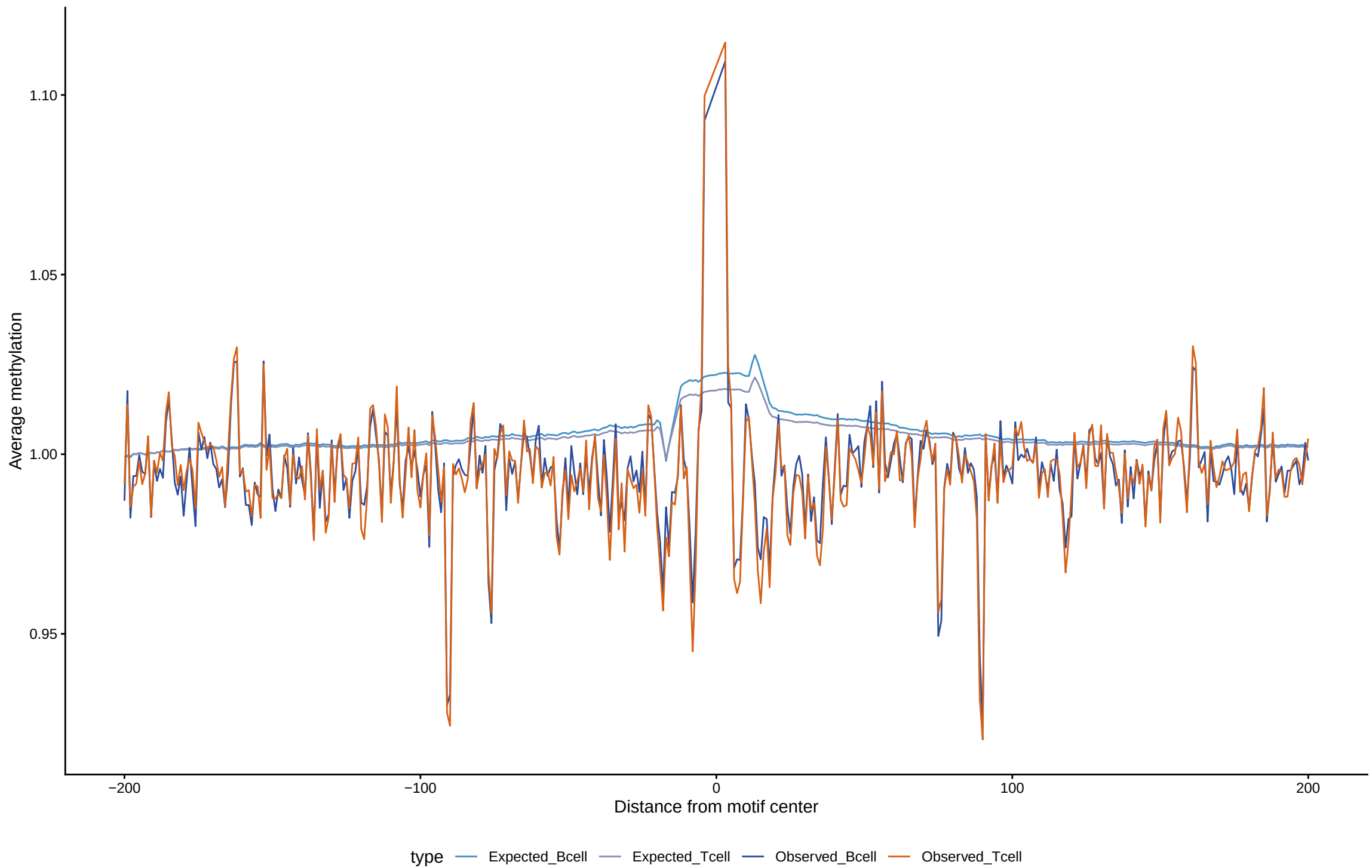
Expected vs observed footprints for MSX2
