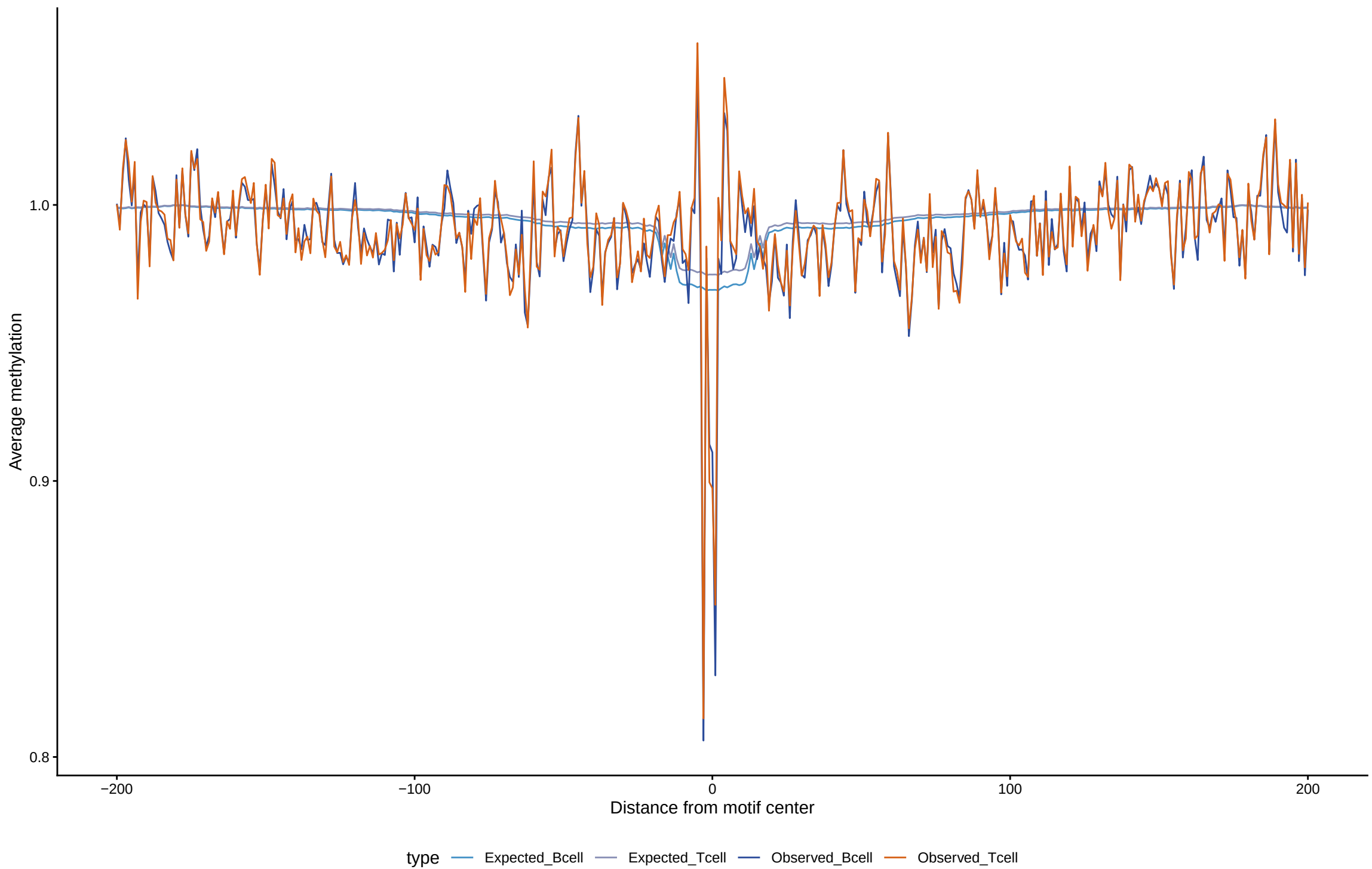
Expected vs observed footprints for MYCN
