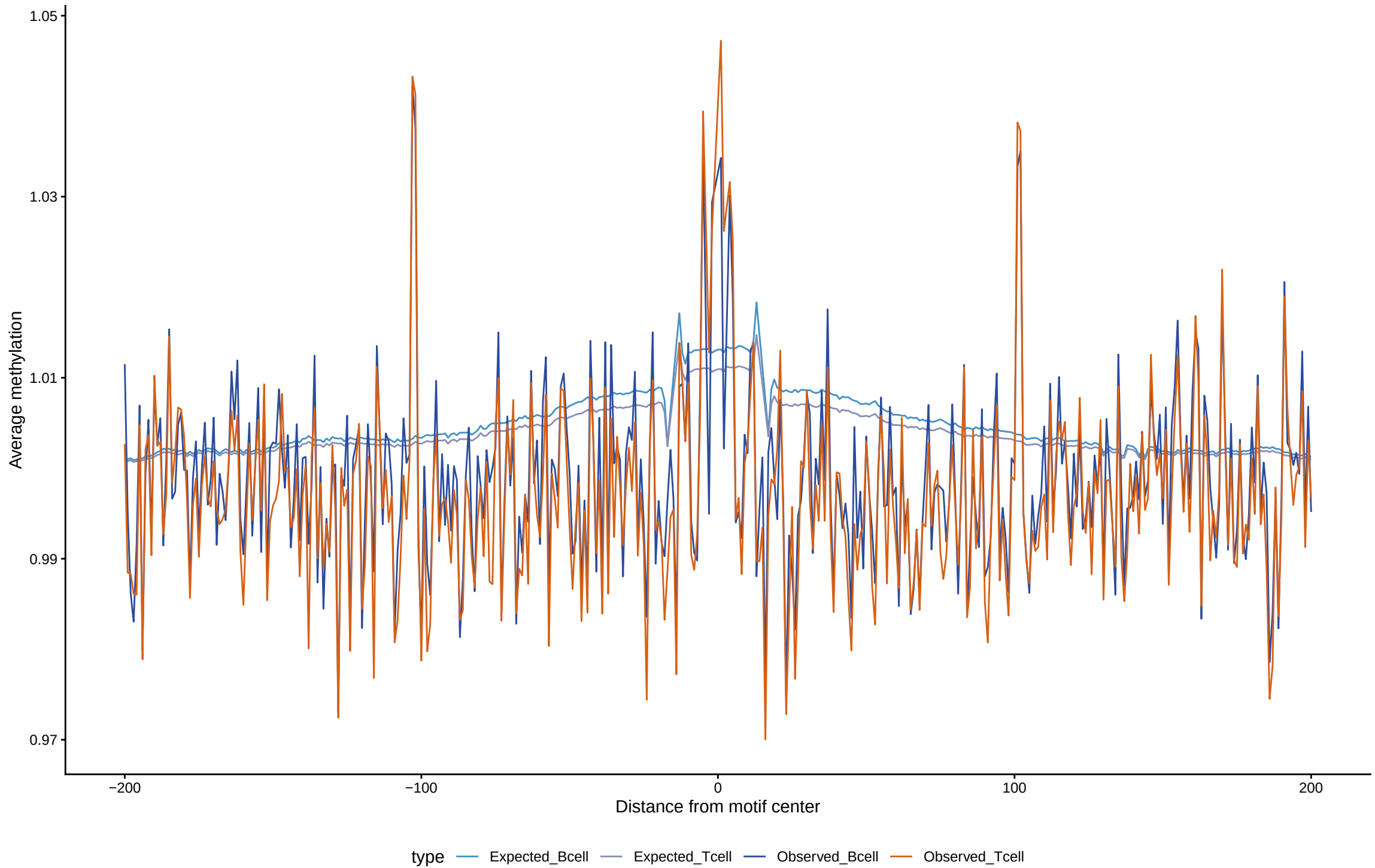
Expected vs observed footprints for NEUROD2
