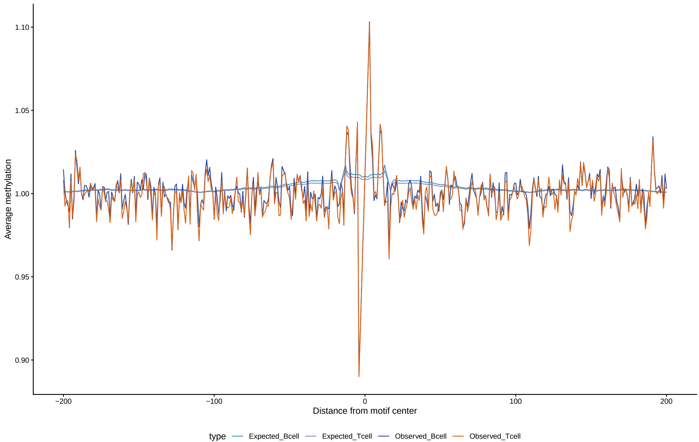
Expected vs observed footprints for NEUROG1
