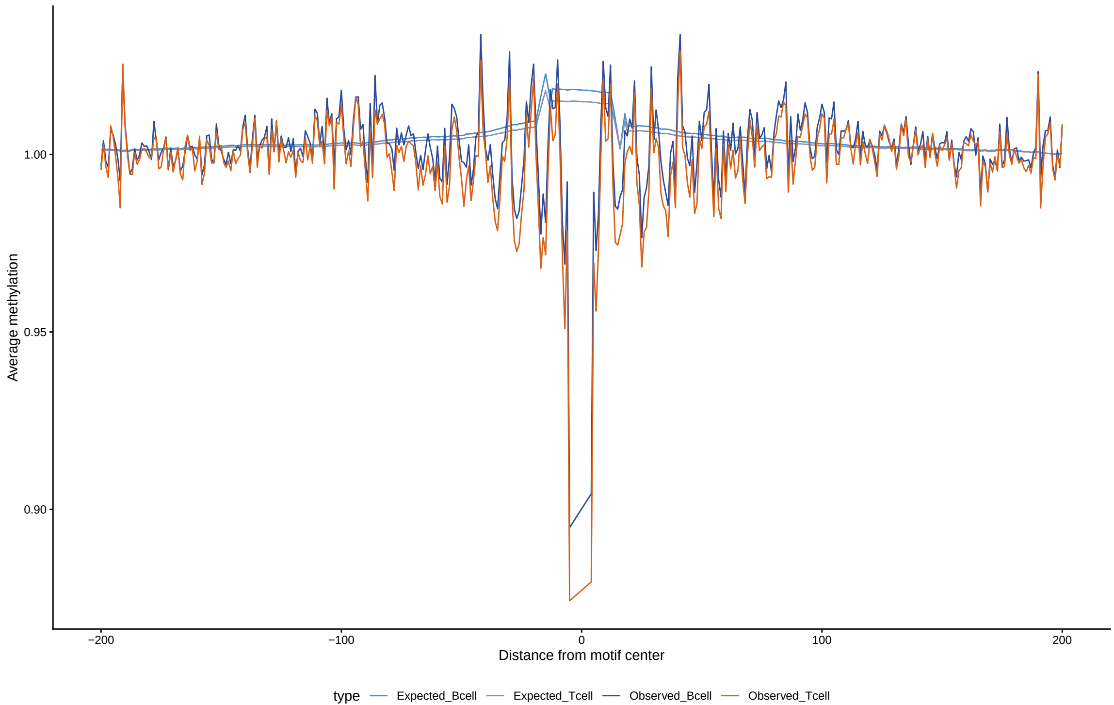
Expected vs observed footprints for NFATC2
