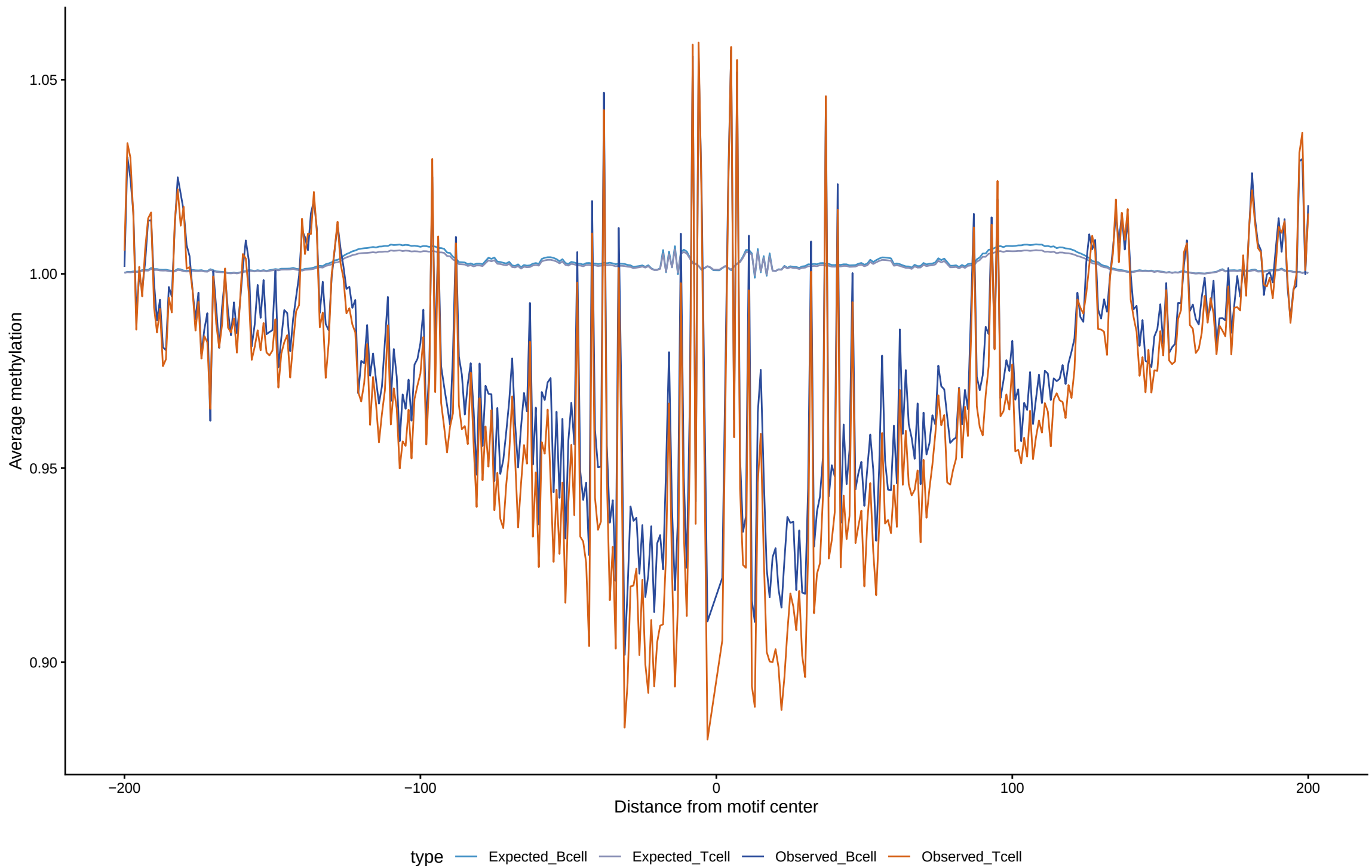
Expected vs observed footprints for NFE2
