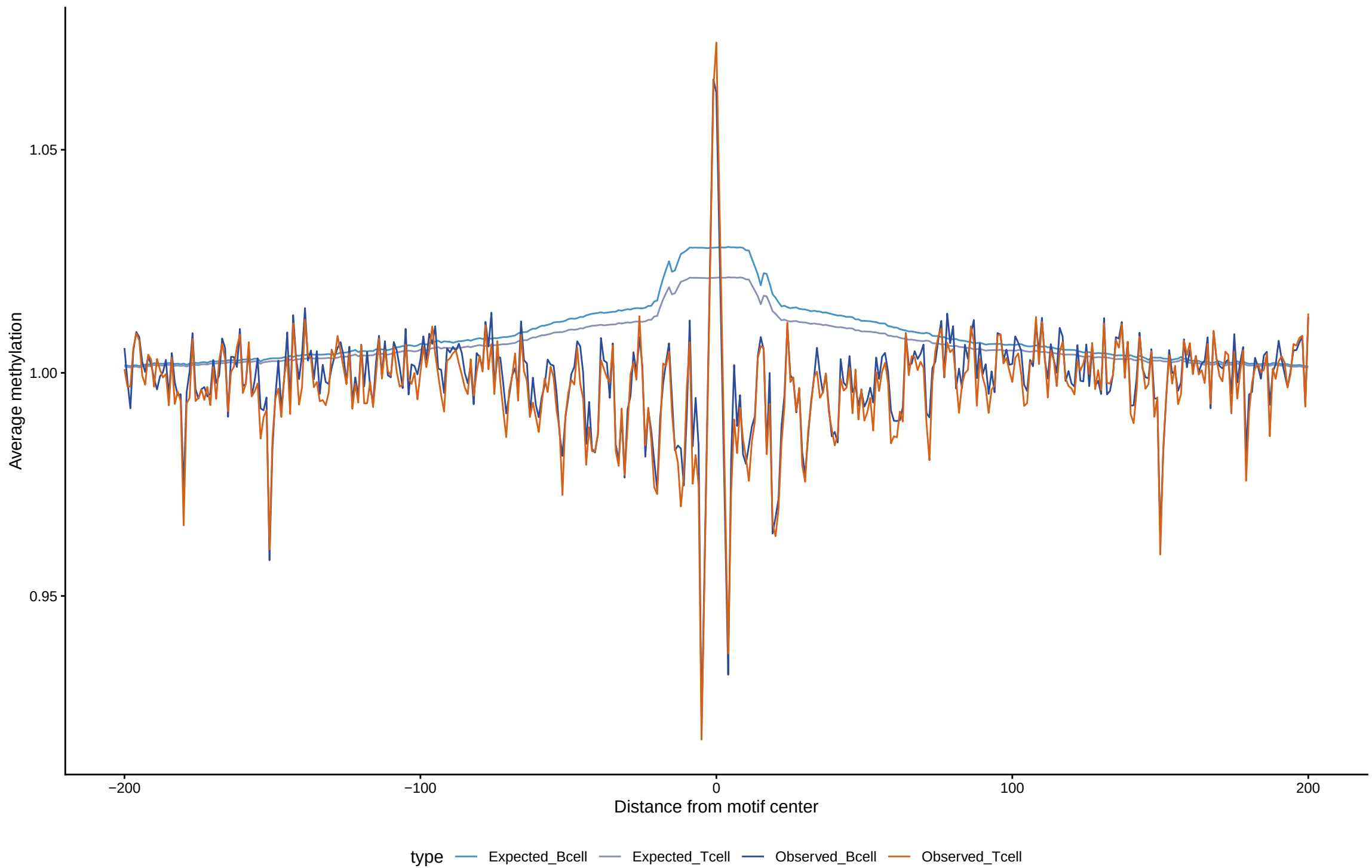
Expected vs observed footprints for NFIL3
