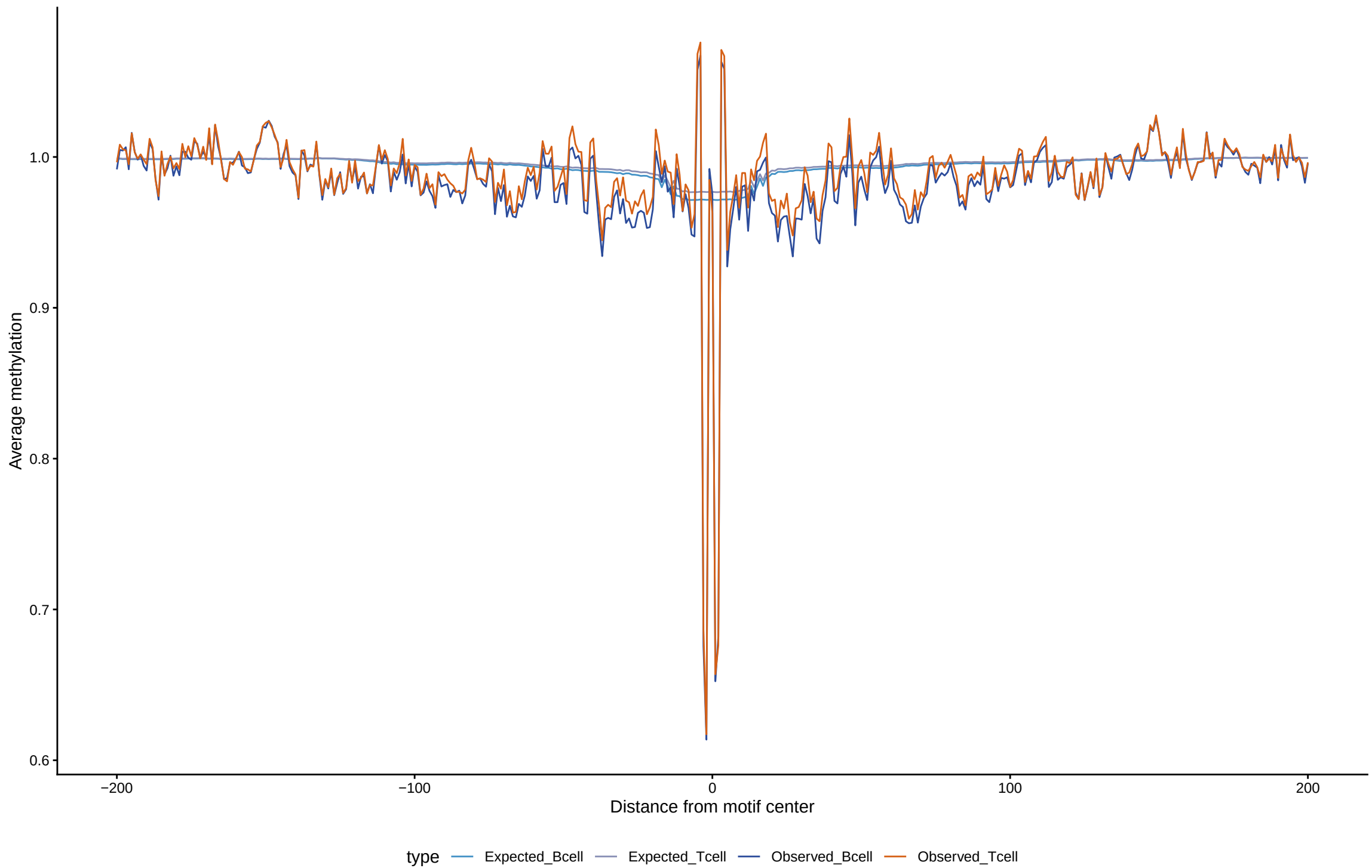
Expected vs observed footprints for NHLH2
