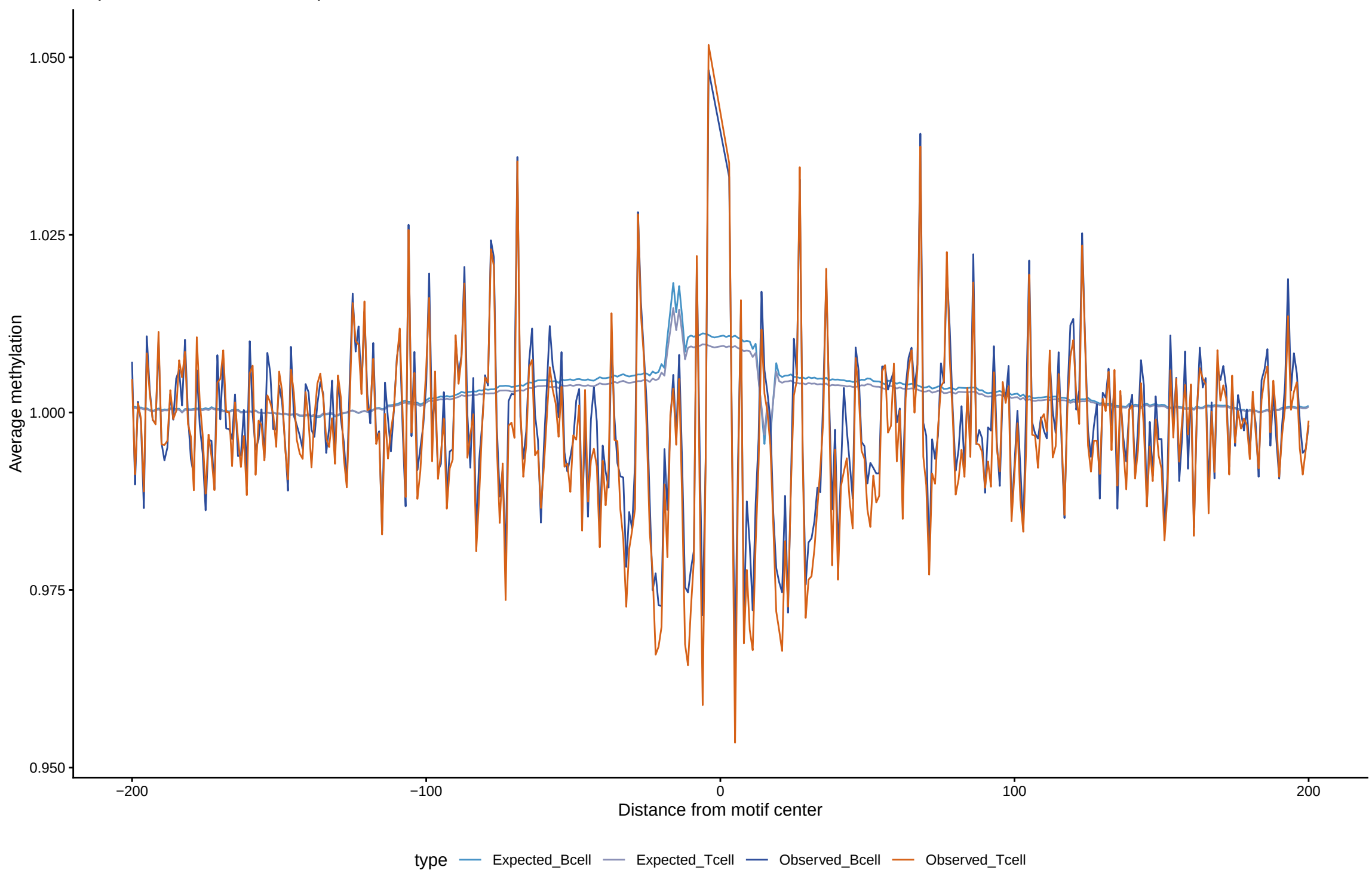
Expected vs observed footprints for NR1H4
