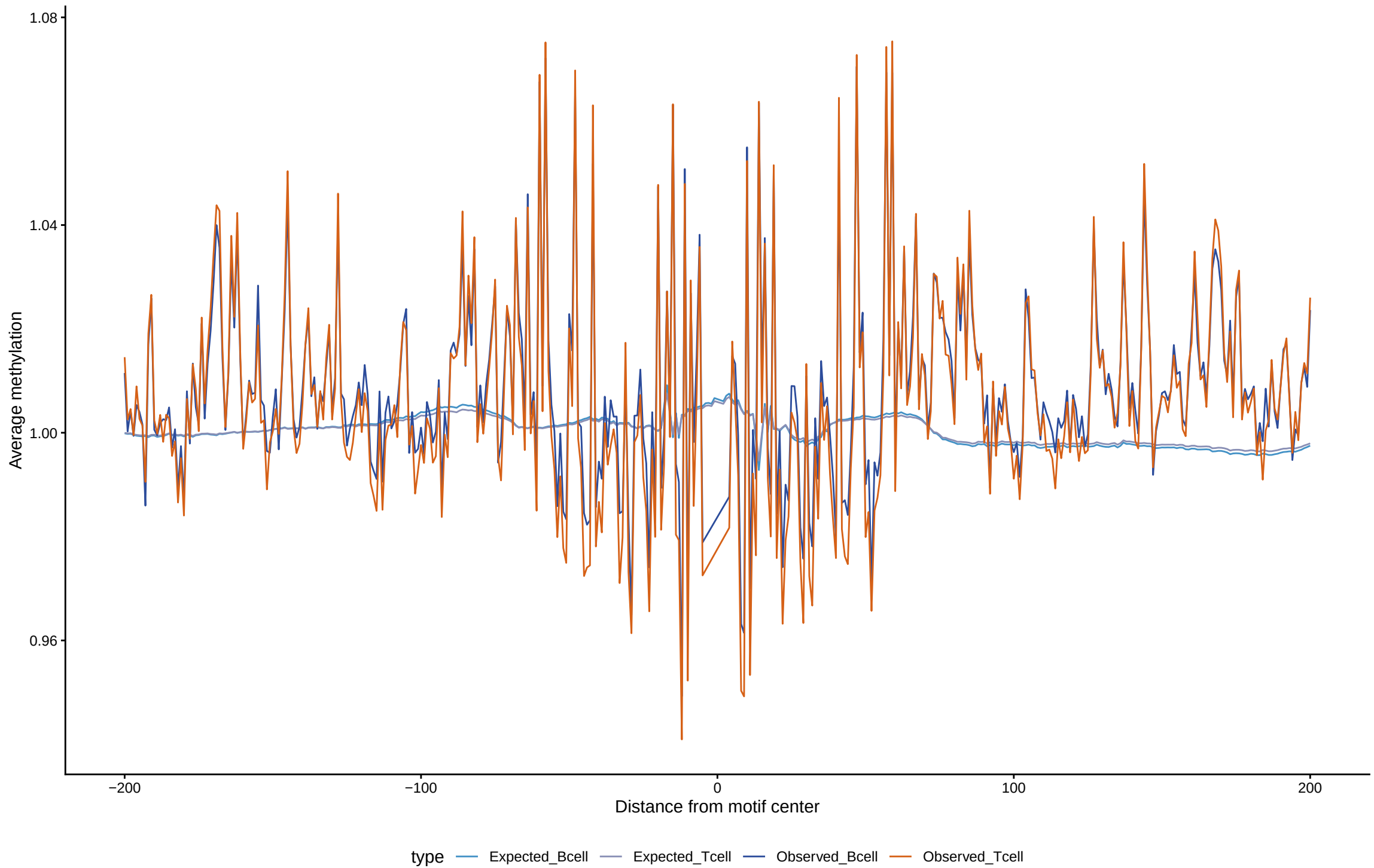
Expected vs observed footprints for NR2F2
