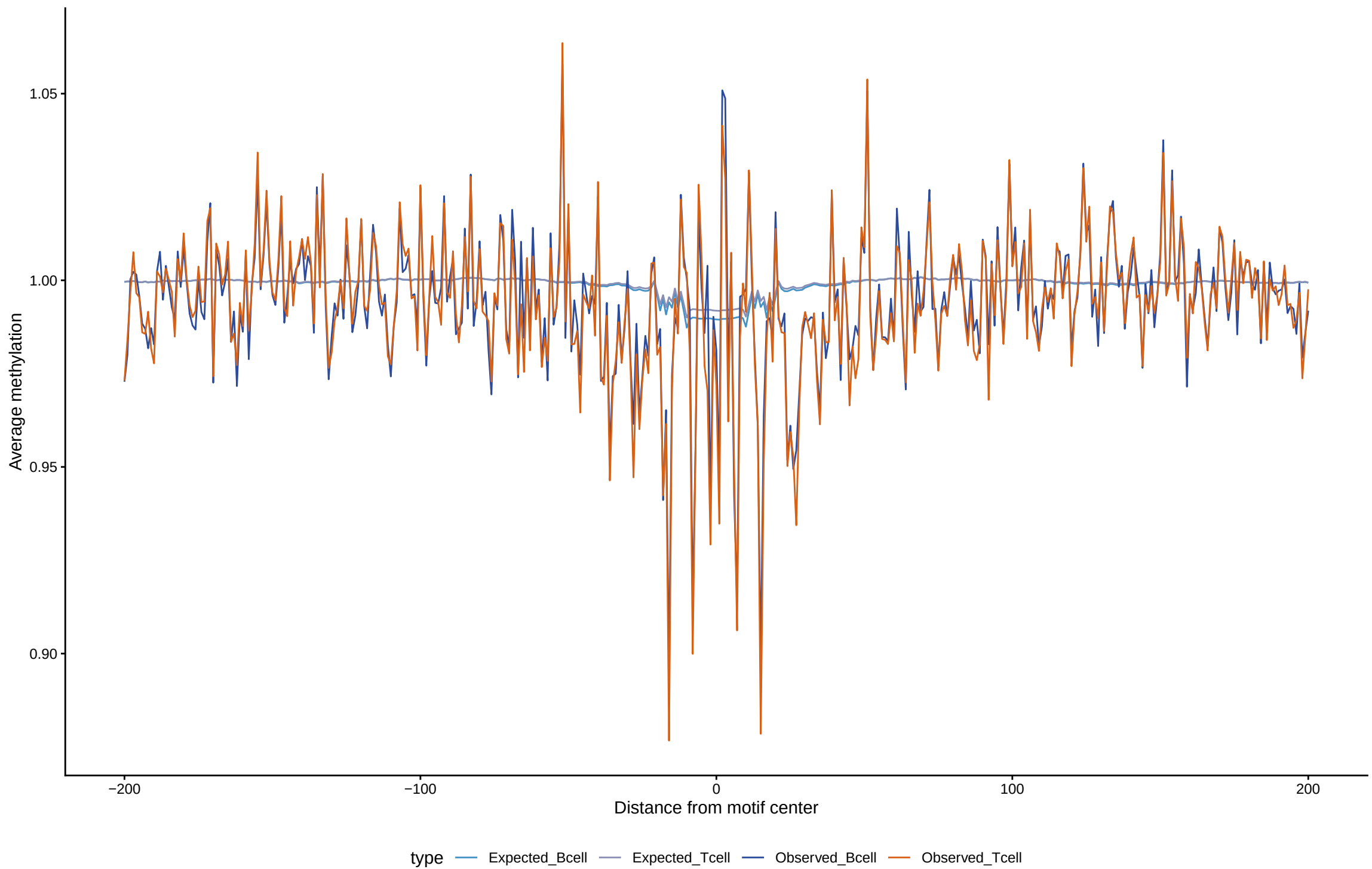
Expected vs observed footprints for NR2F6(var.3)
