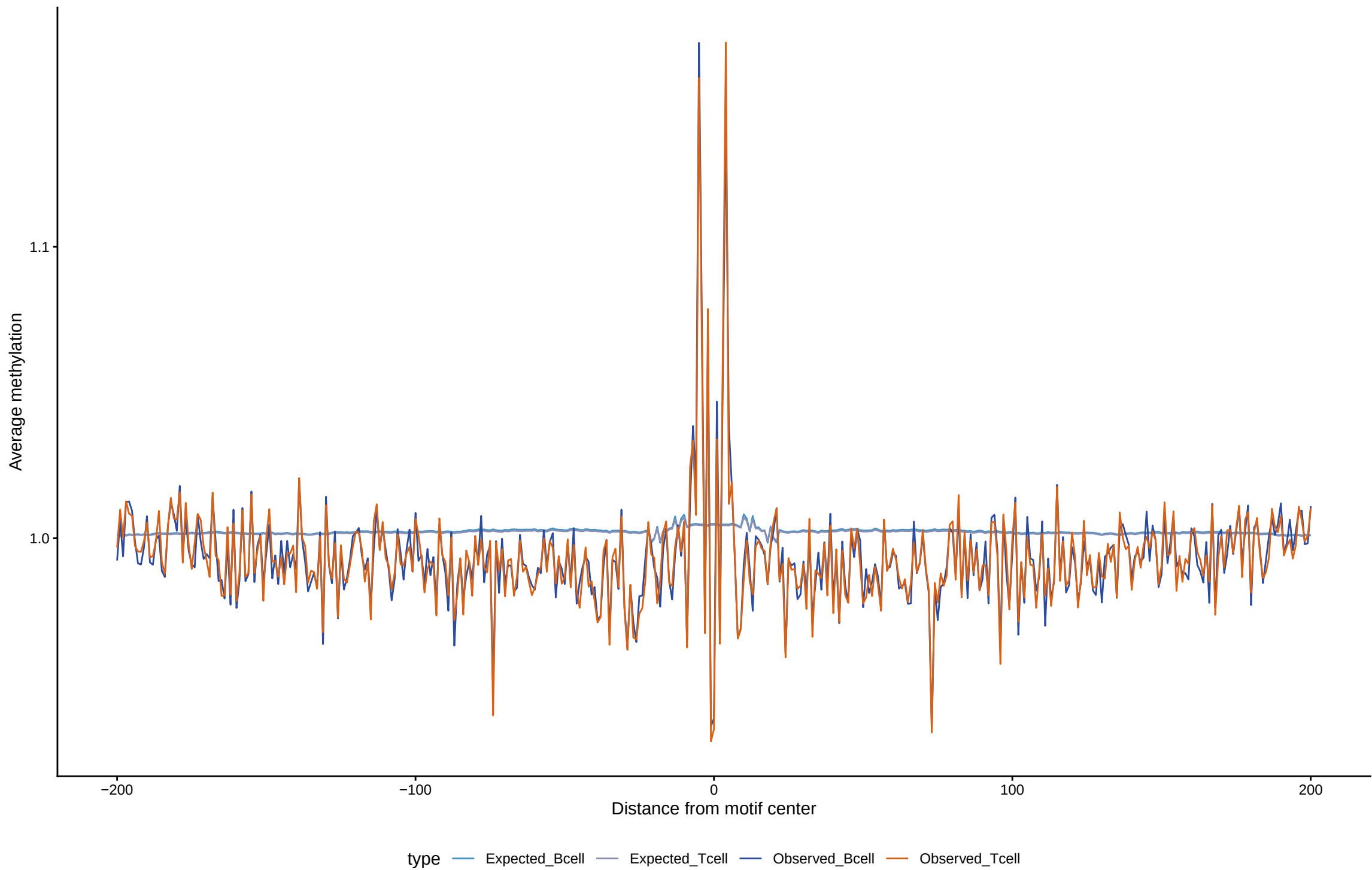
Expected vs observed footprints for NR3C2
