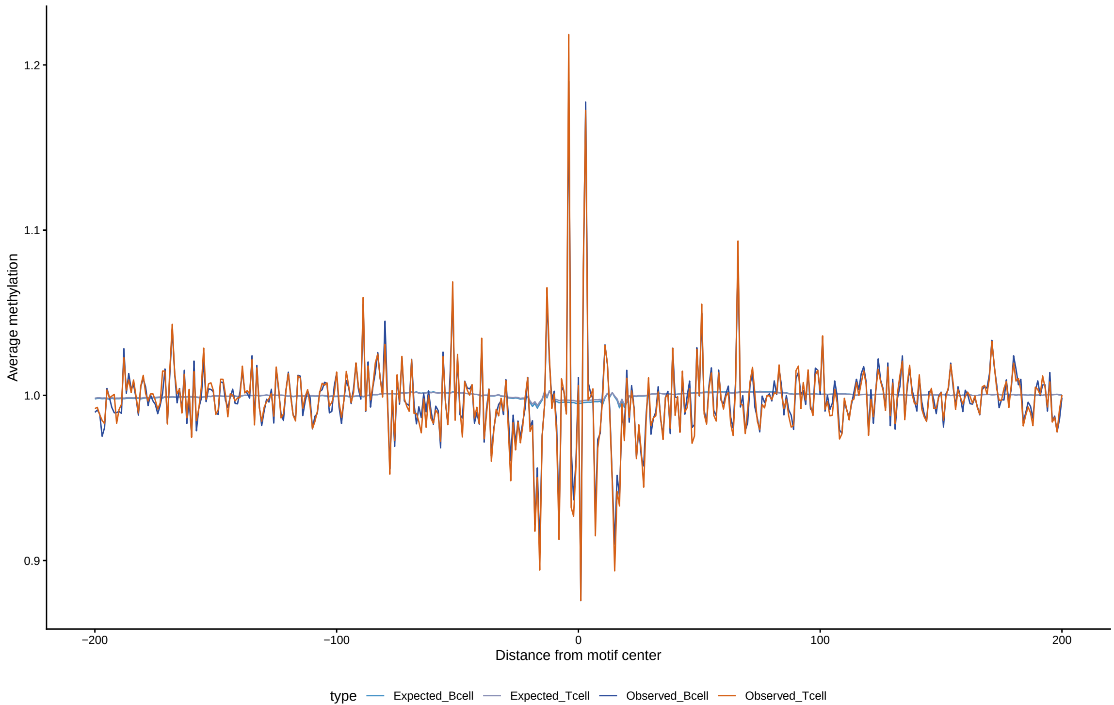
Expected vs observed footprints for NR4A2::RXRA
