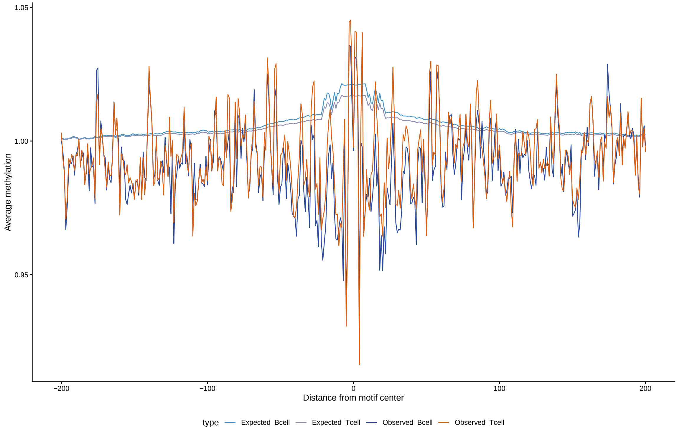
Expected vs observed footprints for PAX6
